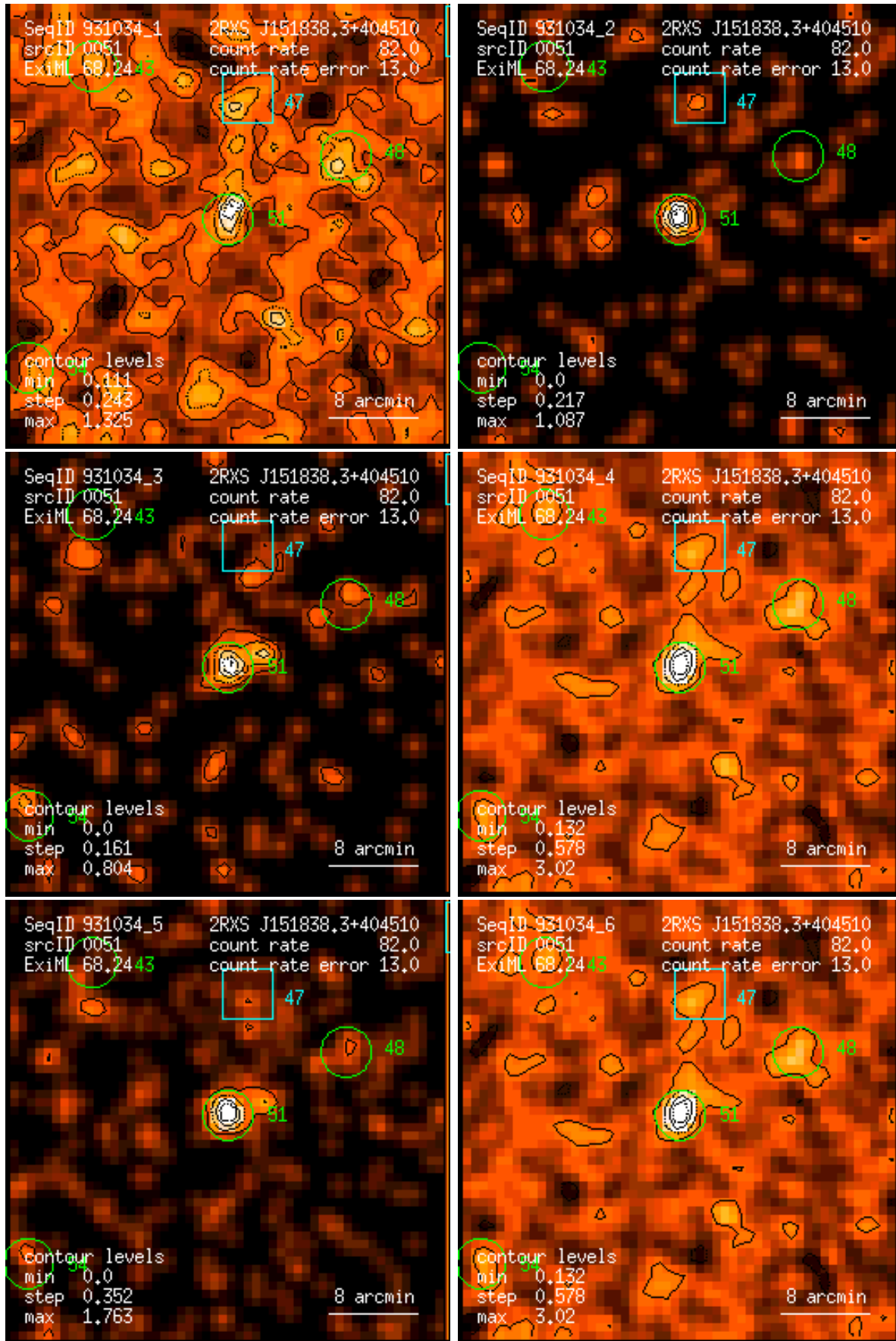
Figure 51: RASS 931034: detection 0051: band rate images, Gaussian filter: (1) PSPC channels 11 – 41, (2) 52 – 90, (3) 91 – 201, (4) 11 – 235, (5) 52 – 201, (6) 11 – 201. Broad band rates in counts/ks. Band rate contour levels in counts/ks/arcmin 2 .
