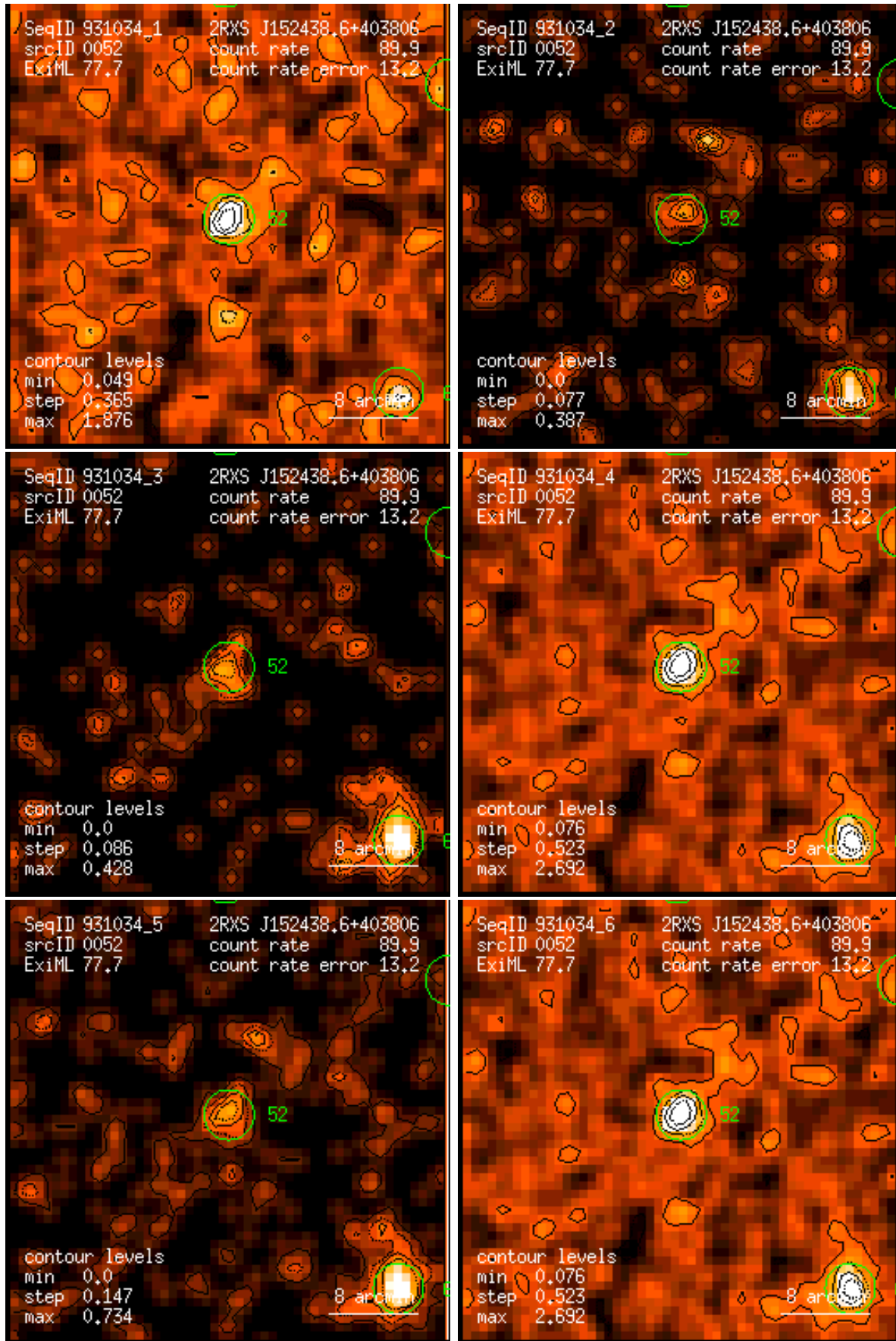
Figure 52: RASS 931034: detection 0052: band rate images, Gaussian filter: (1) PSPC channels 11 – 41, (2) 52 – 90, (3) 91 – 201, (4) 11 – 235, (5) 52 – 201, (6) 11 – 201. Broad band rates in counts/ks. Band rate contour levels in counts/ks/arcmin 2 .
