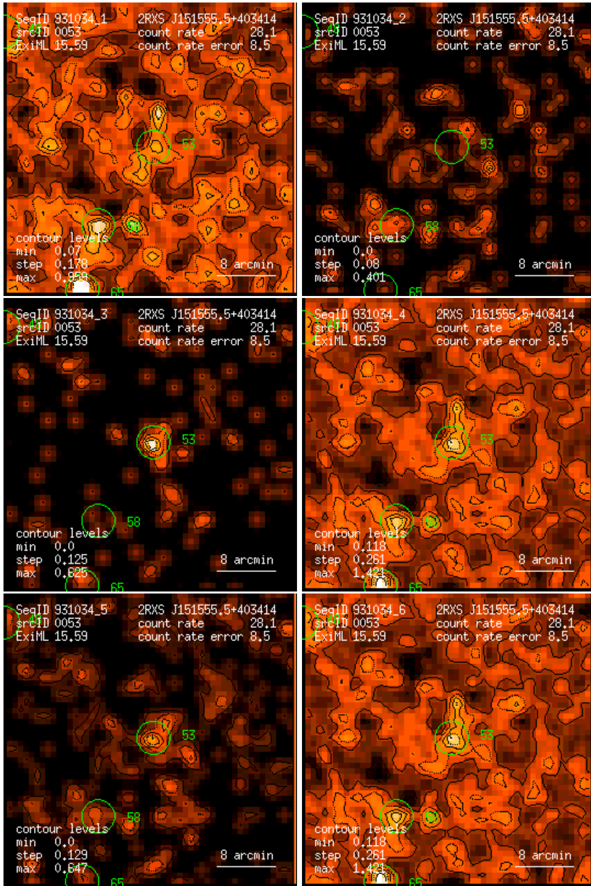
Figure 53: RASS 931034: detection 0053: band rate images, Gaussian filter: (1) PSPC channels 11 – 41, (2) 52 – 90, (3) 91 – 201, (4) 11 – 235, (5) 52 – 201, (6) 11 – 201. Broad band rates in counts/ks. Band rate contour levels in counts/ks/arcmin 2 .
