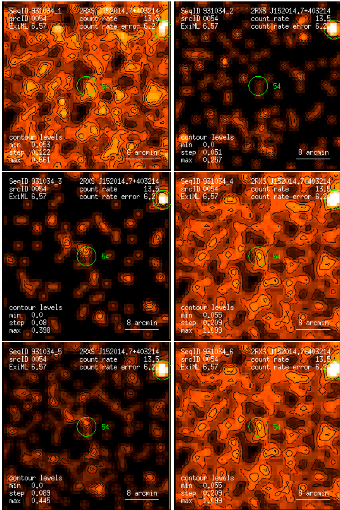
Figure 54: RASS 931034: detection 0054: band rate images, Gaussian filter: (1) PSPC channels 11 – 41, (2) 52 – 90, (3) 91 – 201, (4) 11 – 235, (5) 52 – 201, (6) 11 – 201. Broad band rates in counts/ks. Band rate contour levels in counts/ks/arcmin 2 .
