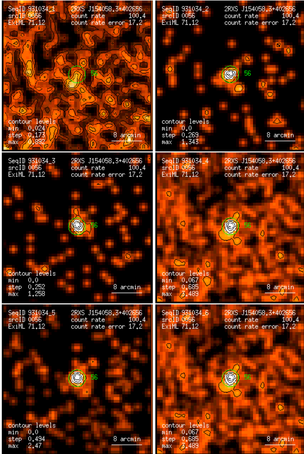
Figure 56: RASS 931034: detection 0056: band rate images, Gaussian filter: (1) PSPC channels 11 – 41, (2) 52 – 90, (3) 91 – 201, (4) 11 – 235, (5) 52 – 201, (6) 11 – 201. Broad band rates in counts/ks. Band rate contour levels in counts/ks/arcmin 2 .
