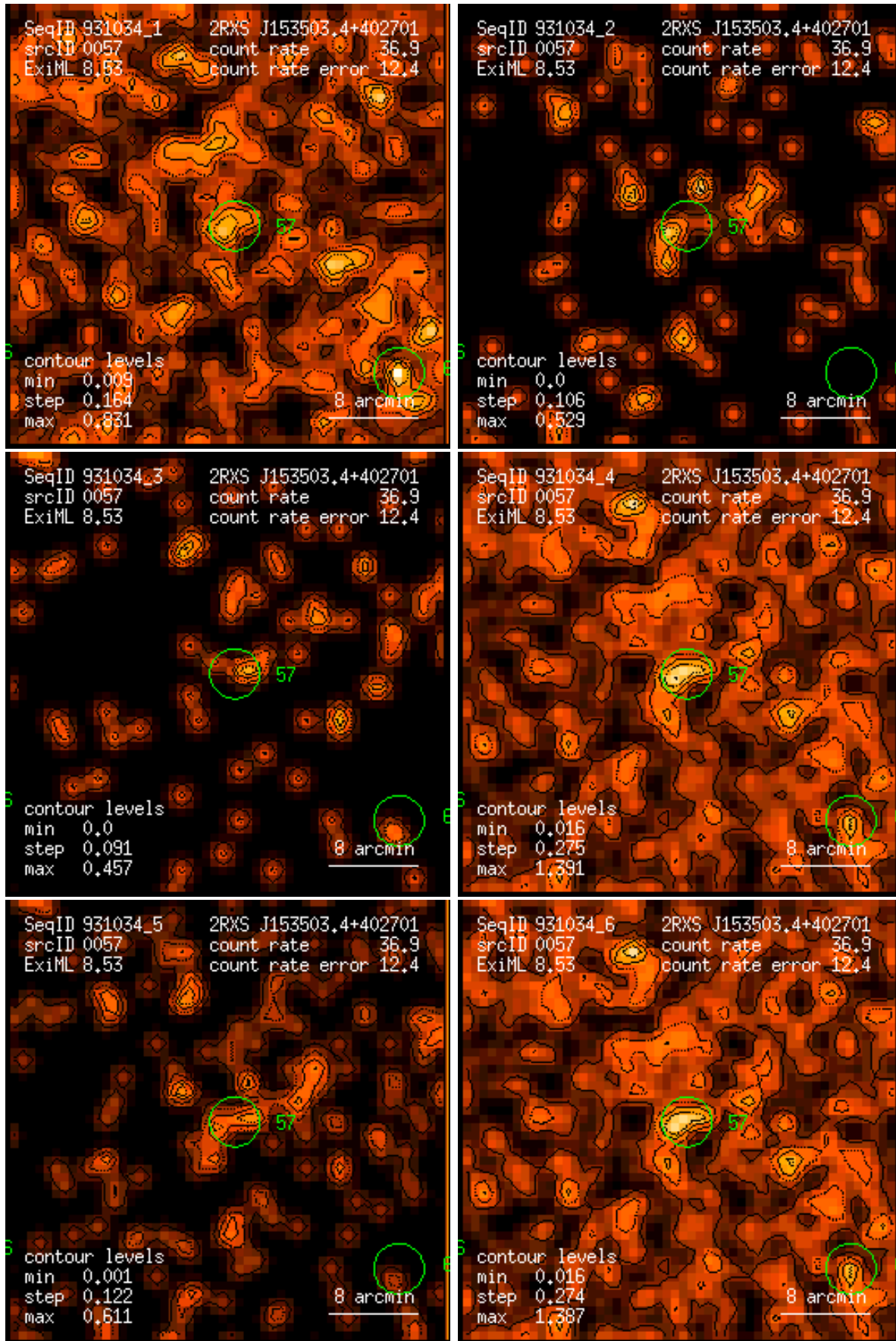
Figure 57: RASS 931034: detection 0057: band rate images, Gaussian filter: (1) PSPC channels 11 – 41, (2) 52 – 90, (3) 91 – 201, (4) 11 – 235, (5) 52 – 201, (6) 11 – 201. Broad band rates in counts/ks. Band rate contour levels in counts/ks/arcmin 2 .
