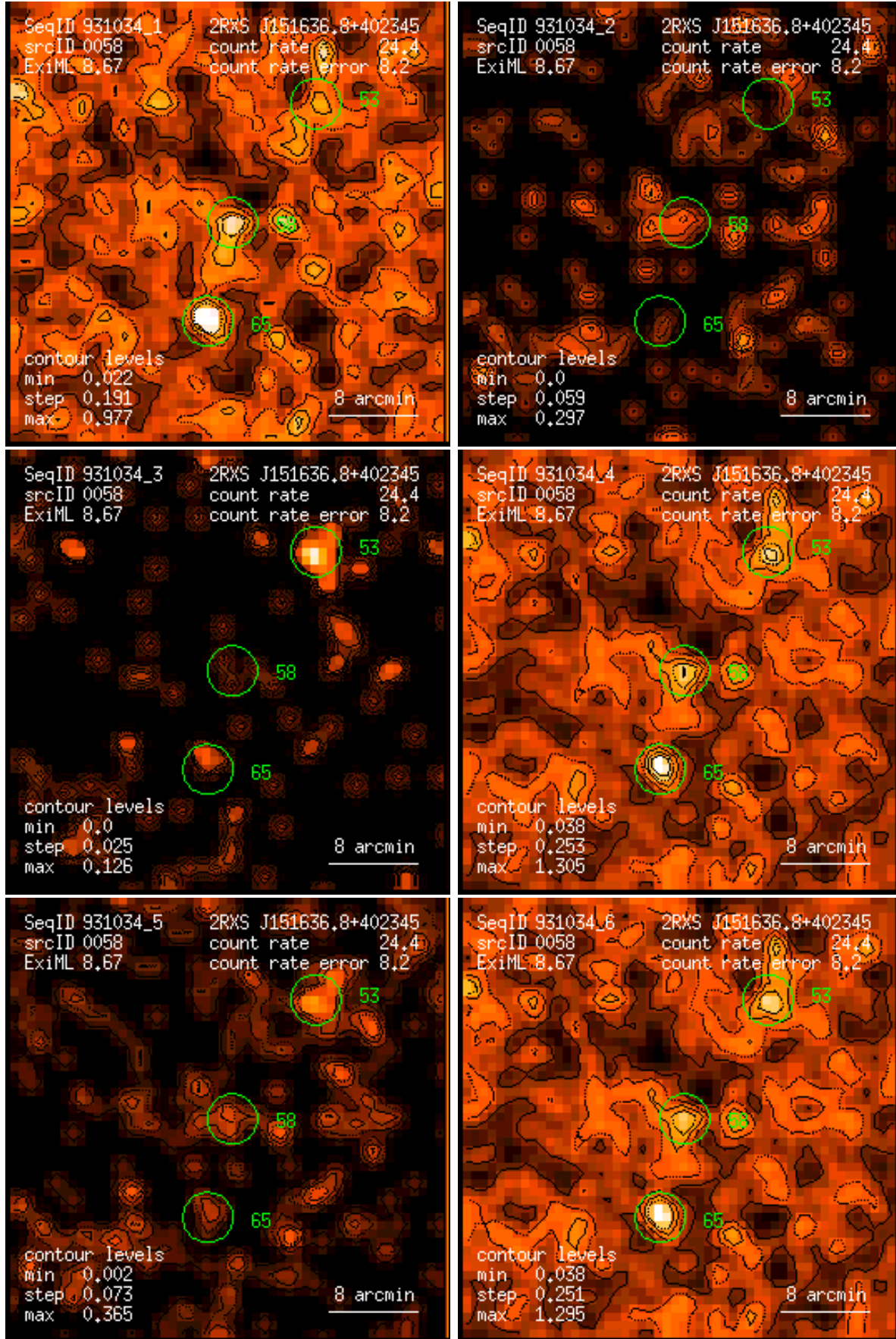
Figure 58: RASS 931034: detection 0058: band rate images, Gaussian filter: (1) PSPC channels 11 – 41, (2) 52 – 90, (3) 91 – 201, (4) 11 – 235, (5) 52 – 201, (6) 11 – 201. Broad band rates in counts/ks. Band rate contour levels in counts/ks/arcmin 2 .
