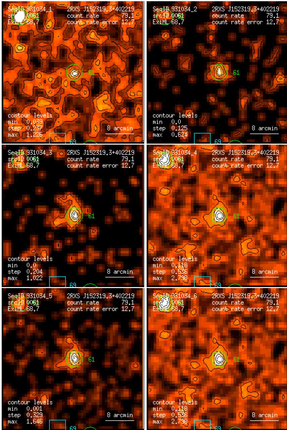
Figure 61: RASS 931034: detection 0061: band rate images, Gaussian filter: (1) PSPC channels 11 – 41, (2) 52 – 90, (3) 91 – 201, (4) 11 – 235, (5) 52 – 201, (6) 11 – 201. Broad band rates in counts/ks. Band rate contour levels in counts/ks/arcmin 2 .
