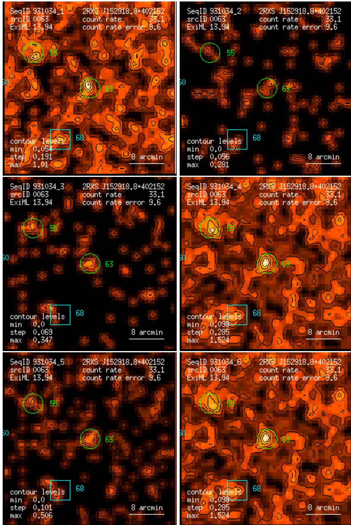
Figure 63: RASS 931034: detection 0063: band rate images, Gaussian filter: (1) PSPC channels 11 – 41, (2) 52 – 90, (3) 91 – 201, (4) 11 – 235, (5) 52 – 201, (6) 11 – 201. Broad band rates in counts/ks. Band rate contour levels in counts/ks/arcmin 2 .
