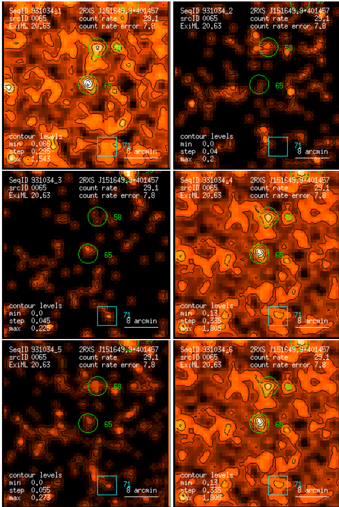
Figure 65: RASS 931034: detection 0065: band rate images, Gaussian filter: (1) PSPC channels 11 – 41, (2) 52 – 90, (3) 91 – 201, (4) 11 – 235, (5) 52 – 201, (6) 11 – 201. Broad band rates in counts/ks. Band rate contour levels in counts/ks/arcmin 2 .
