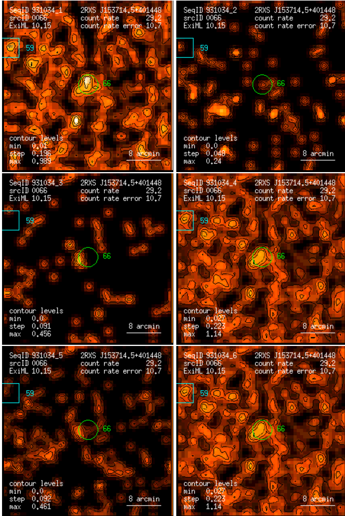
Figure 66: RASS 931034: detection 0066: band rate images, Gaussian filter: (1) PSPC channels 11 – 41, (2) 52 – 90, (3) 91 – 201, (4) 11 – 235, (5) 52 – 201, (6) 11 – 201. Broad band rates in counts/ks. Band rate contour levels in counts/ks/arcmin 2 .
