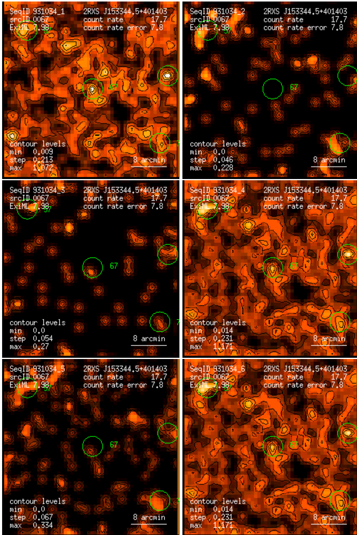
Figure 67: RASS 931034: detection 0067: band rate images, Gaussian filter: (1) PSPC channels 11 – 41, (2) 52 – 90, (3) 91 – 201, (4) 11 – 235, (5) 52 – 201, (6) 11 – 201. Broad band rates in counts/ks. Band rate contour levels in counts/ks/arcmin 2 .
