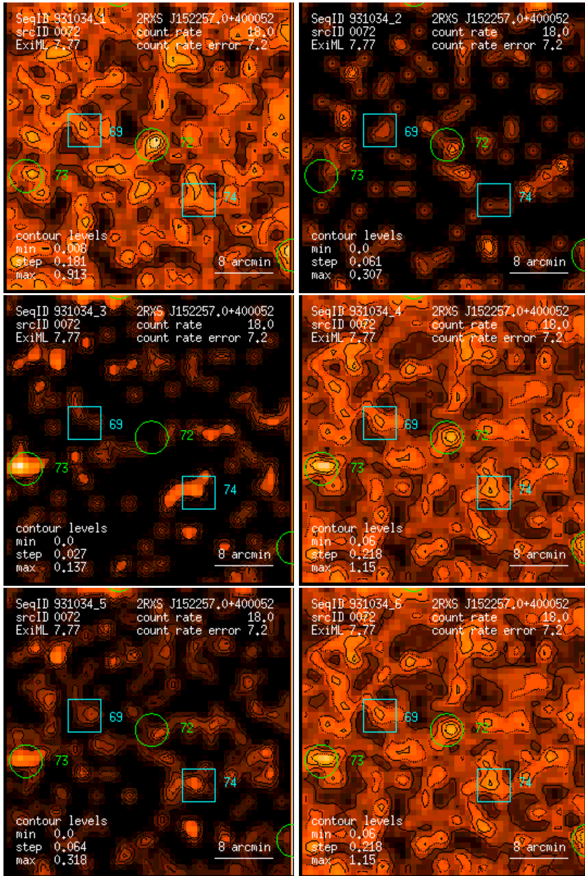
Figure 72: RASS 931034: detection 0072: band rate images, Gaussian filter: (1) PSPC channels 11 – 41, (2) 52 – 90, (3) 91 – 201, (4) 11 – 235, (5) 52 – 201, (6) 11 – 201. Broad band rates in counts/ks. Band rate contour levels in counts/ks/arcmin 2 .
