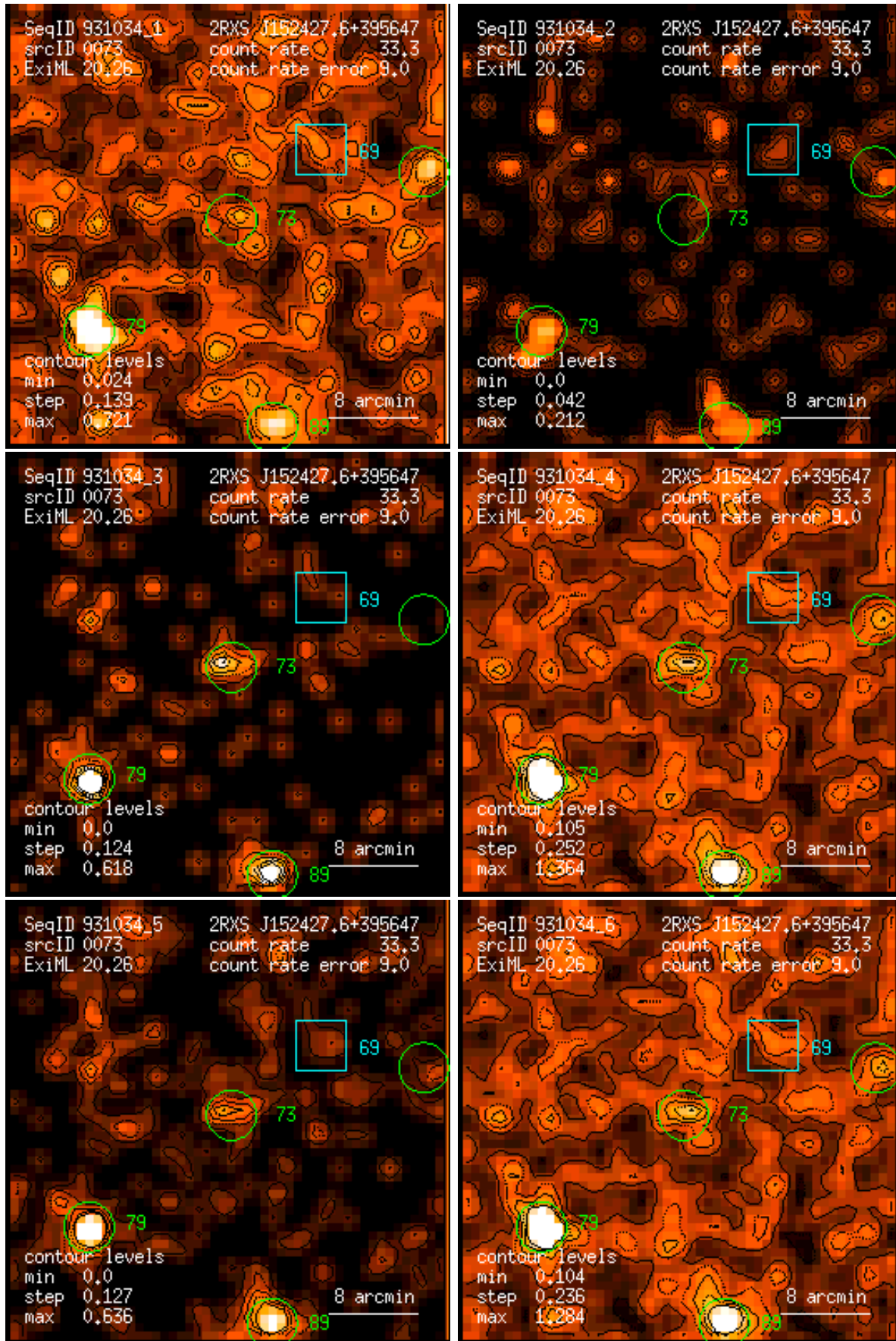
Figure 73: RASS 931034: detection 0073: band rate images, Gaussian filter: (1) PSPC channels 11 – 41, (2) 52 – 90, (3) 91 – 201, (4) 11 – 235, (5) 52 – 201, (6) 11 – 201. Broad band rates in counts/ks. Band rate contour levels in counts/ks/arcmin 2 .
