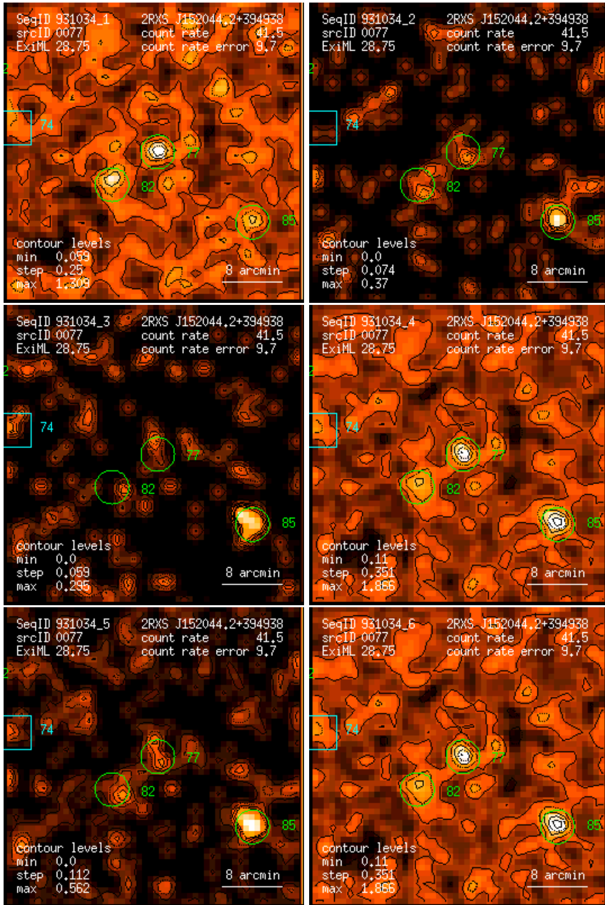
Figure 77: RASS 931034: detection 0077: band rate images, Gaussian filter: (1) PSPC channels 11 – 41, (2) 52 – 90, (3) 91 – 201, (4) 11 – 235, (5) 52 – 201, (6) 11 – 201. Broad band rates in counts/ks. Band rate contour levels in counts/ks/arcmin 2 .
