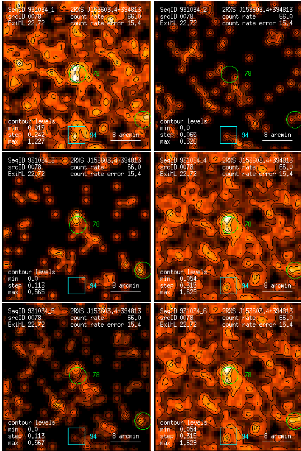
Figure 78: RASS 931034: detection 0078: band rate images, Gaussian filter: (1) PSPC channels 11 – 41, (2) 52 – 90, (3) 91 – 201, (4) 11 – 235, (5) 52 – 201, (6) 11 – 201. Broad band rates in counts/ks. Band rate contour levels in counts/ks/arcmin 2 .
