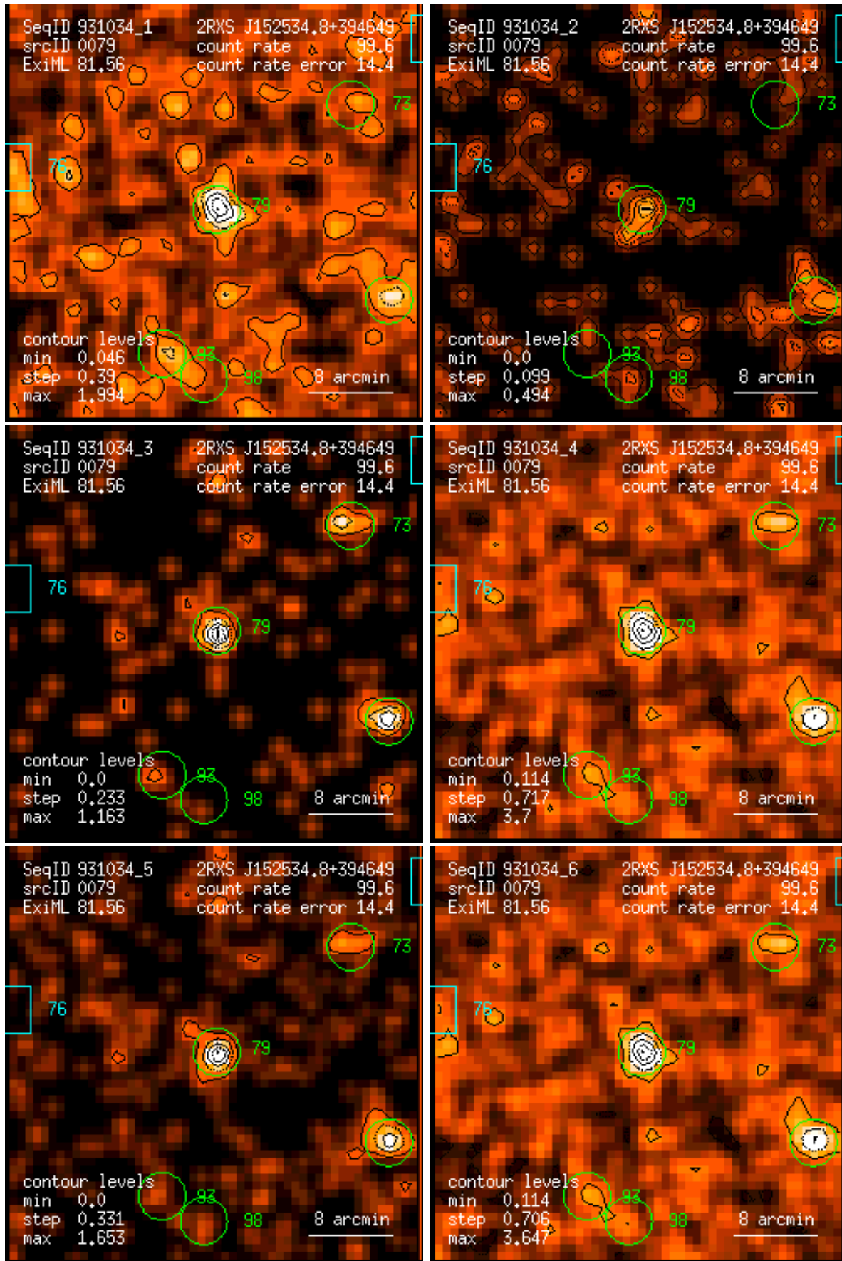
Figure 79: RASS 931034: detection 0079: band rate images, Gaussian filter: (1) PSPC channels 11 – 41, (2) 52 – 90, (3) 91 – 201, (4) 11 – 235, (5) 52 – 201, (6) 11 – 201. Broad band rates in counts/ks. Band rate contour levels in counts/ks/arcmin 2 .
