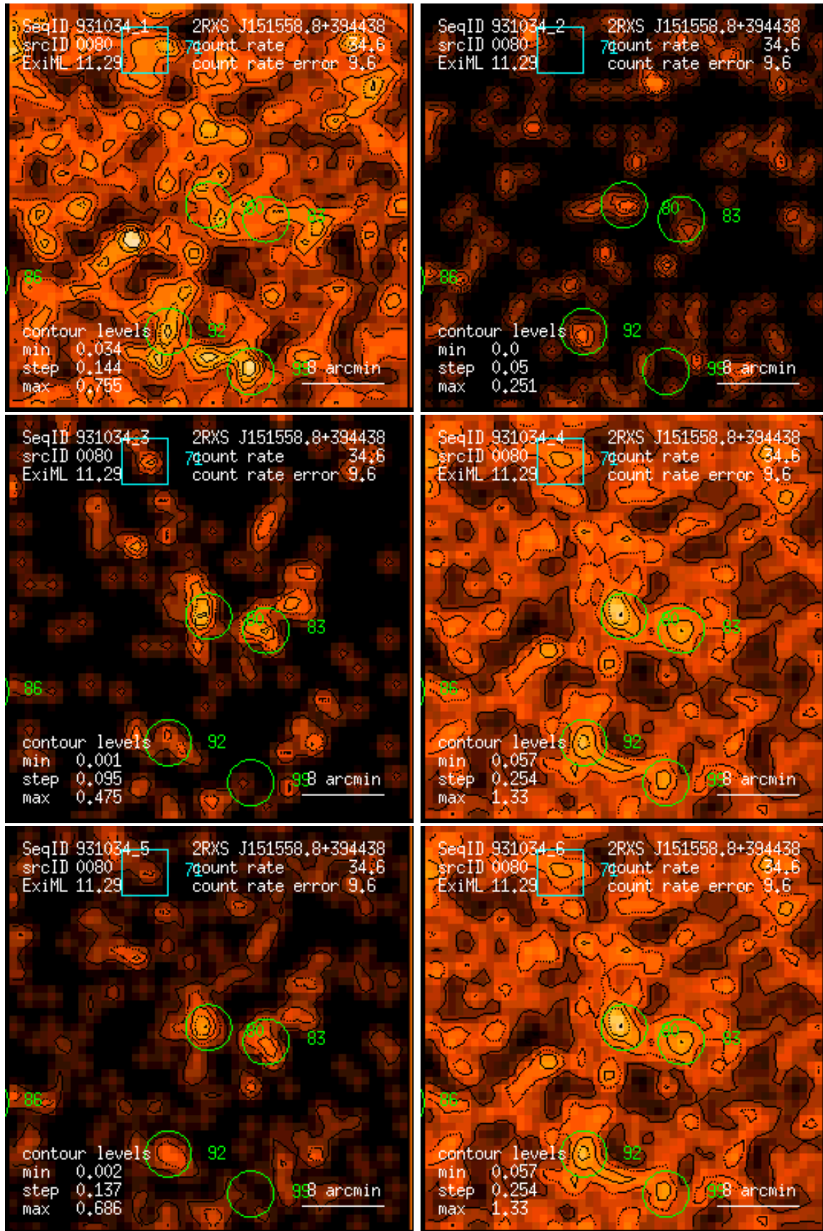
Figure 80: RASS 931034: detection 0080: band rate images, Gaussian filter: (1) PSPC channels 11 – 41, (2) 52 – 90, (3) 91 – 201, (4) 11 – 235, (5) 52 – 201, (6) 11 – 201. Broad band rates in counts/ks. Band rate contour levels in counts/ks/arcmin 2 .
