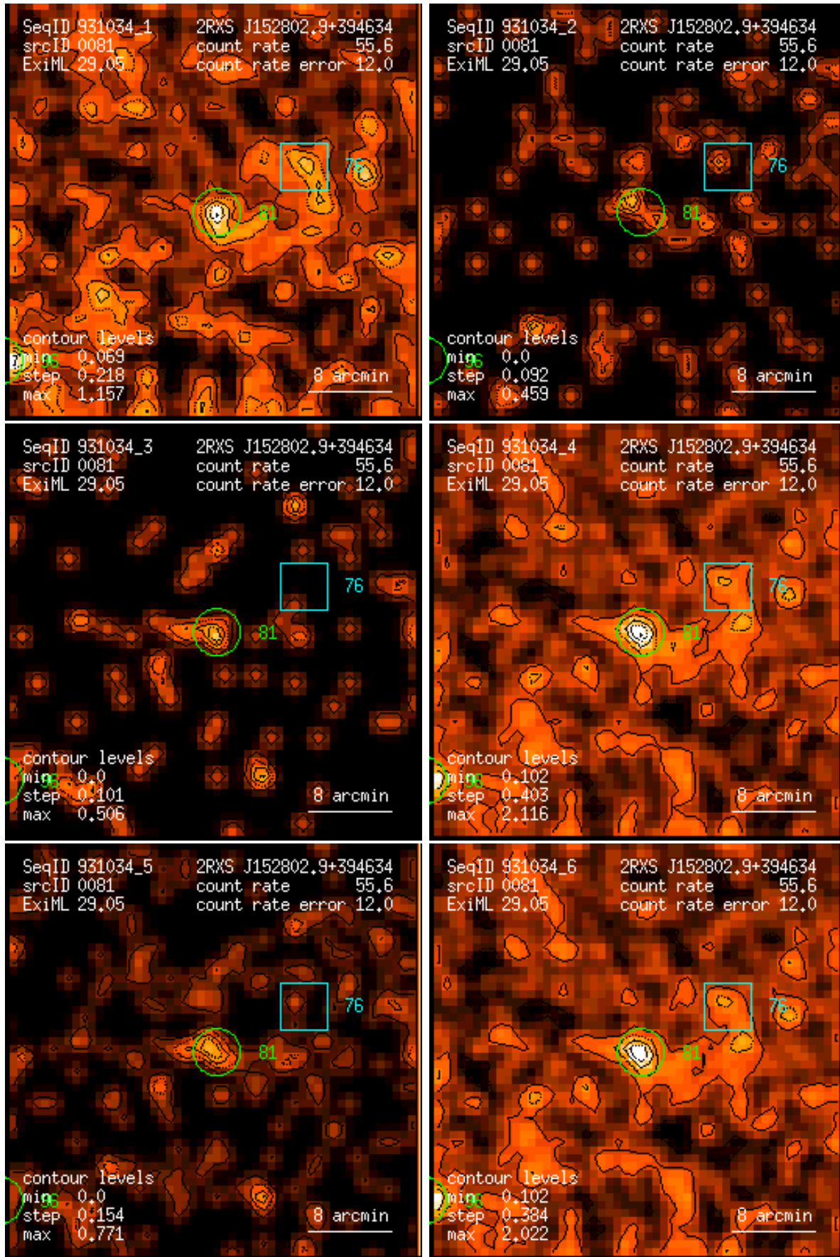
Figure 81: RASS 931034: detection 0081: band rate images, Gaussian filter: (1) PSPC channels 11 – 41, (2) 52 – 90, (3) 91 – 201, (4) 11 – 235, (5) 52 – 201, (6) 11 – 201. Broad band rates in counts/ks. Band rate contour levels in counts/ks/arcmin 2 .
