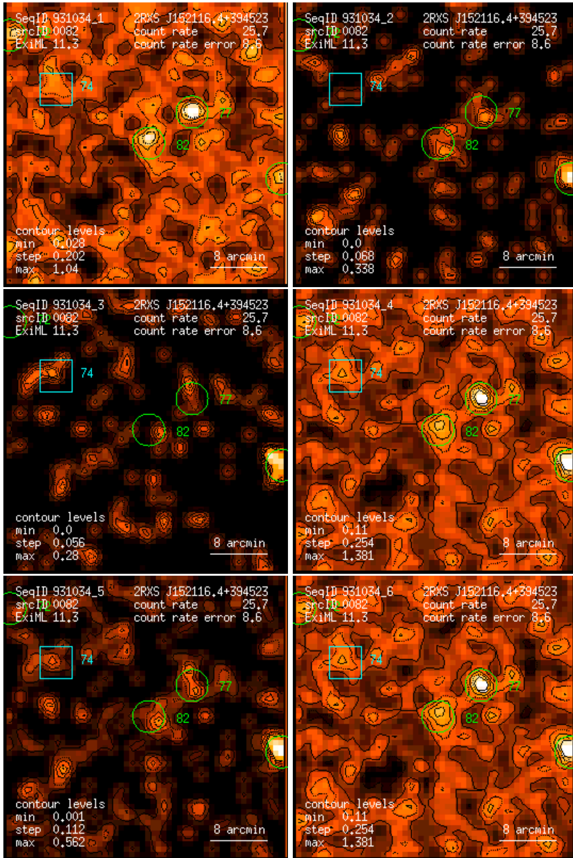
Figure 82: RASS 931034: detection 0082: band rate images, Gaussian filter: (1) PSPC channels 11 – 41, (2) 52 – 90, (3) 91 – 201, (4) 11 – 235, (5) 52 – 201, (6) 11 – 201. Broad band rates in counts/ks. Band rate contour levels in counts/ks/arcmin 2 .
