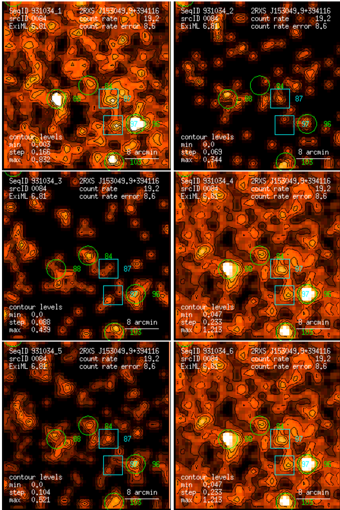
Figure 84: RASS 931034: detection 0084: band rate images, Gaussian filter: (1) PSPC channels 11 – 41, (2) 52 – 90, (3) 91 – 201, (4) 11 – 235, (5) 52 – 201, (6) 11 – 201. Broad band rates in counts/ks. Band rate contour levels in counts/ks/arcmin 2 .
