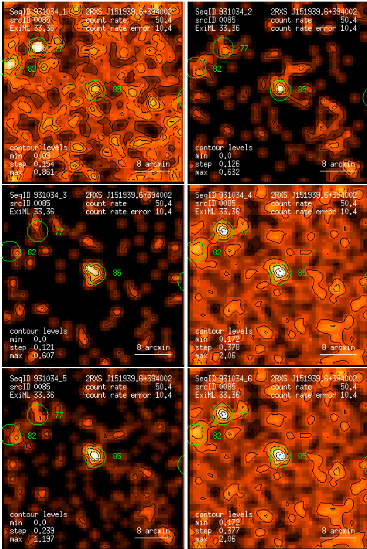
Figure 85: RASS 931034: detection 0085: band rate images, Gaussian filter: (1) PSPC channels 11 – 41, (2) 52 – 90, (3) 91 – 201, (4) 11 – 235, (5) 52 – 201, (6) 11 – 201. Broad band rates in counts/ks. Band rate contour levels in counts/ks/arcmin 2 .
