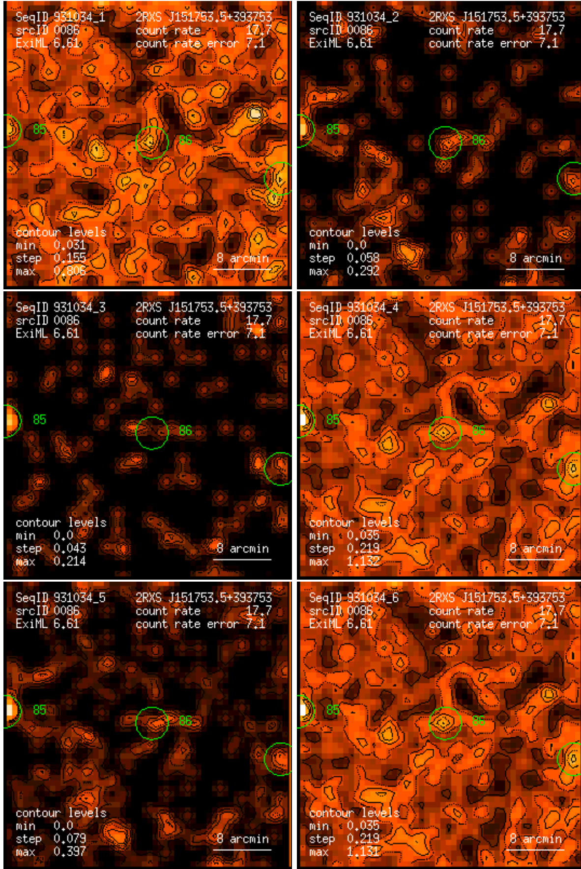
Figure 86: RASS 931034: detection 0086: band rate images, Gaussian filter: (1) PSPC channels 11 – 41, (2) 52 – 90, (3) 91 – 201, (4) 11 – 235, (5) 52 – 201, (6) 11 – 201. Broad band rates in counts/ks. Band rate contour levels in counts/ks/arcmin 2 .
