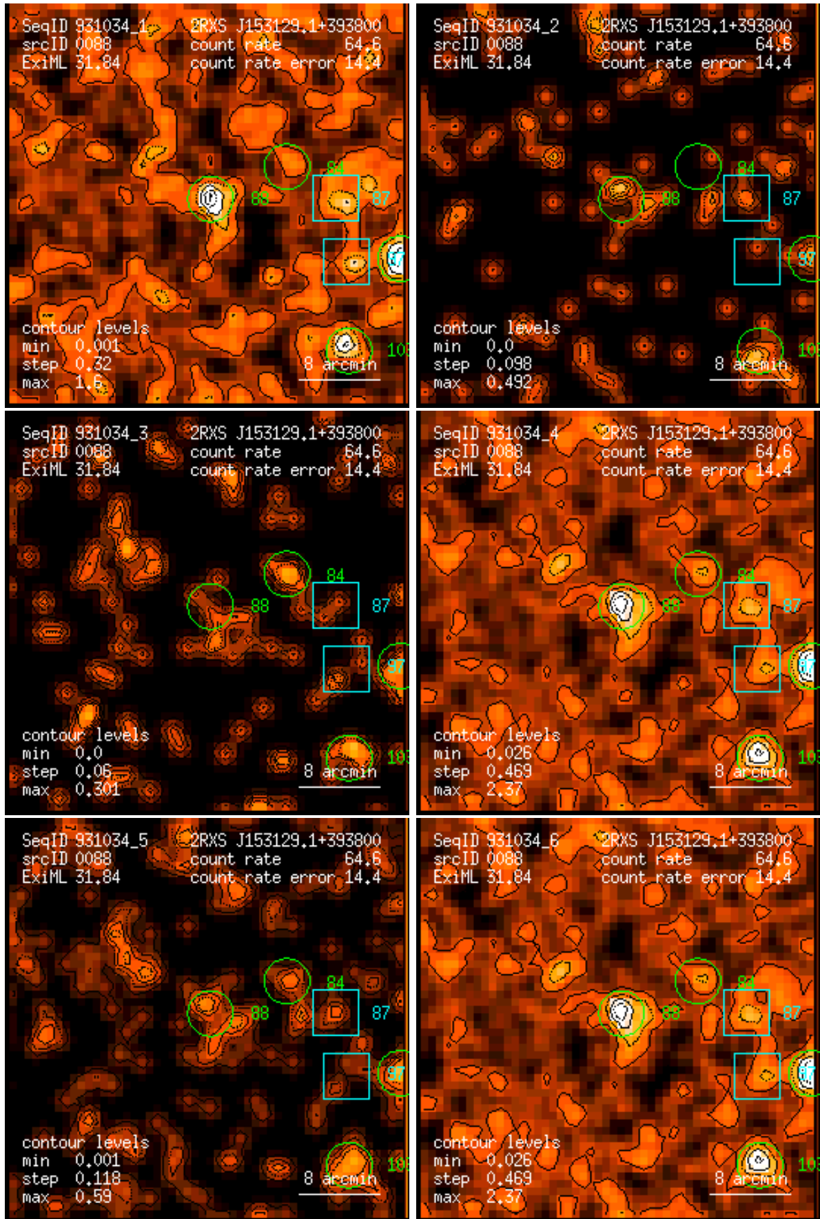
Figure 88: RASS 931034: detection 0088: band rate images, Gaussian filter: (1) PSPC channels 11 – 41, (2) 52 – 90, (3) 91 – 201, (4) 11 – 235, (5) 52 – 201, (6) 11 – 201. Broad band rates in counts/ks. Band rate contour levels in counts/ks/arcmin 2 .
