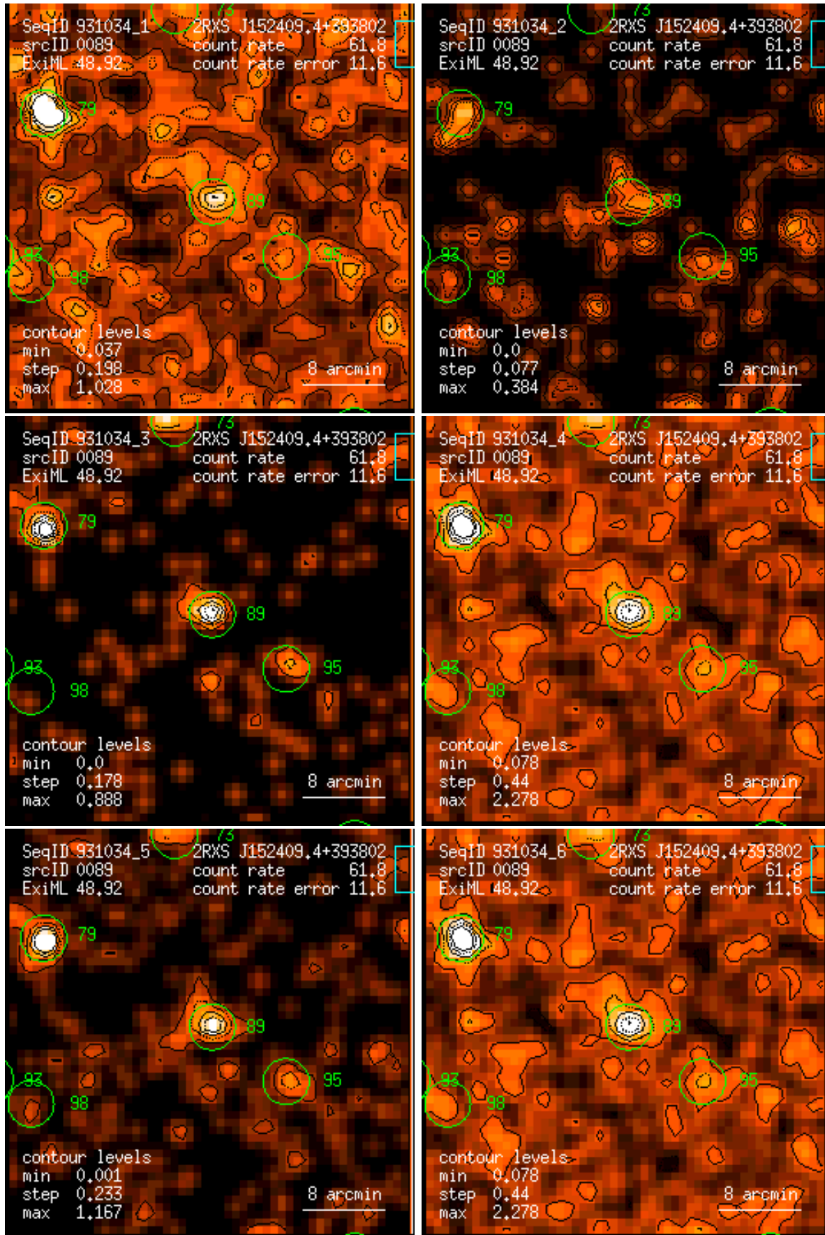
Figure 89: RASS 931034: detection 0089: band rate images, Gaussian filter: (1) PSPC channels 11 – 41, (2) 52 – 90, (3) 91 – 201, (4) 11 – 235, (5) 52 – 201, (6) 11 – 201. Broad band rates in counts/ks. Band rate contour levels in counts/ks/arcmin 2 .
