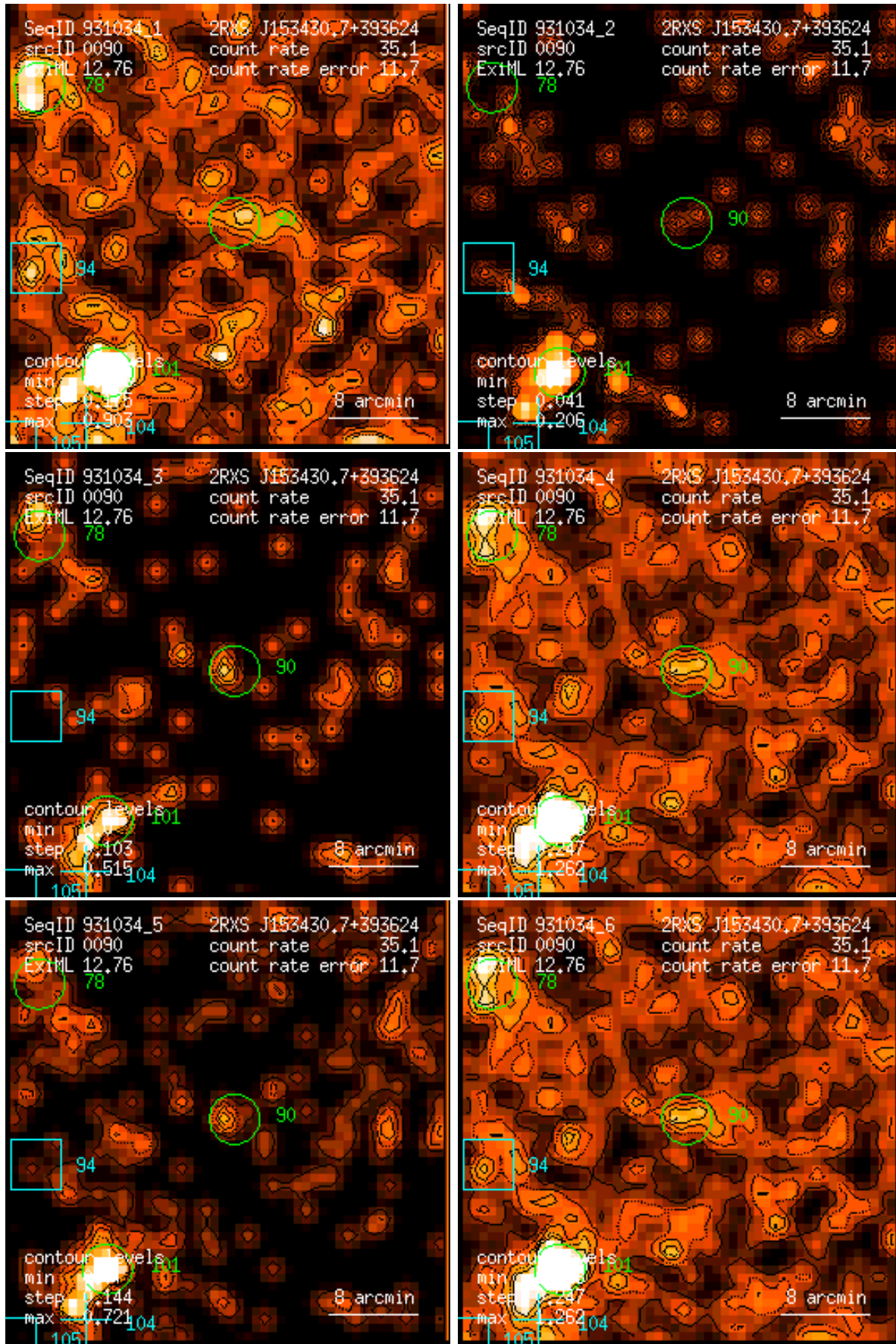
Figure 90: RASS 931034: detection 0090: band rate images, Gaussian filter: (1) PSPC channels 11 – 41, (2) 52 – 90, (3) 91 – 201, (4) 11 – 235, (5) 52 – 201, (6) 11 – 201. Broad band rates in counts/ks. Band rate contour levels in counts/ks/arcmin 2 .
