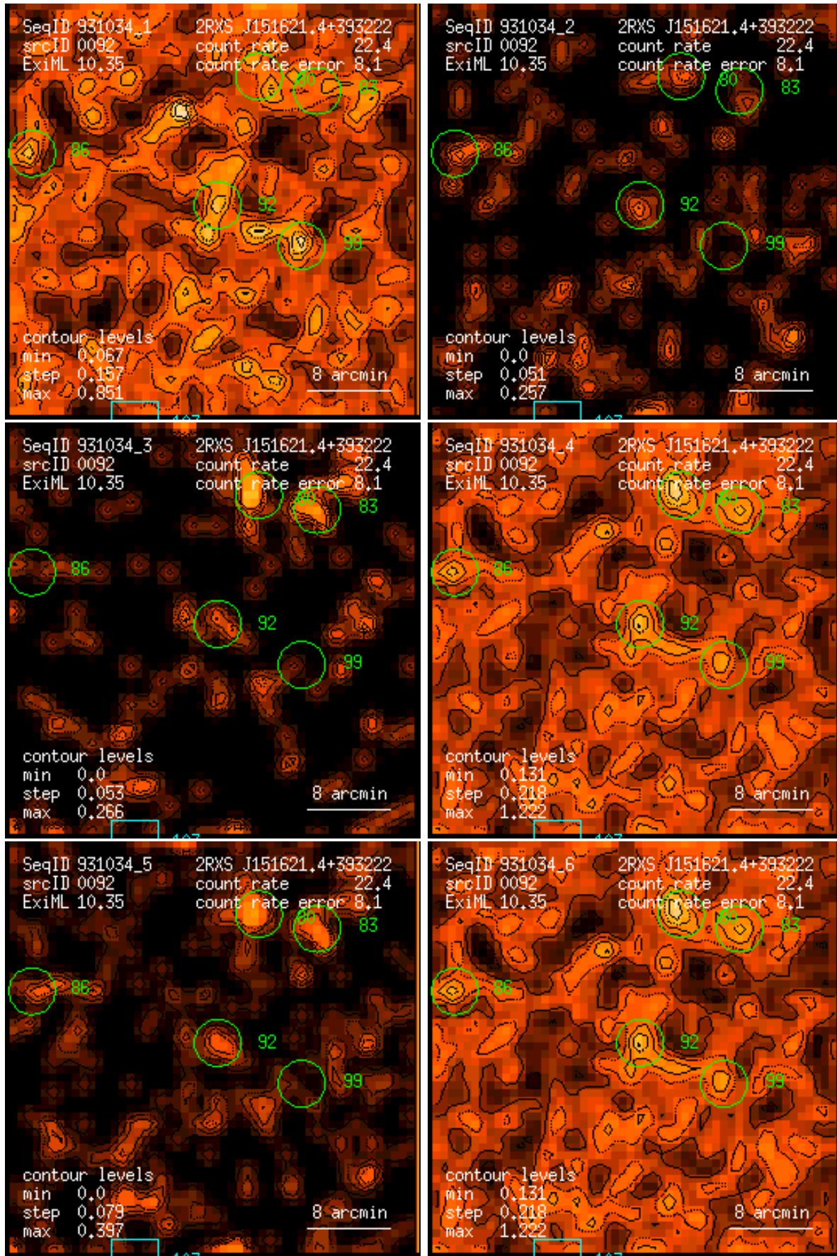
Figure 92: RASS 931034: detection 0092: band rate images, Gaussian filter: (1) PSPC channels 11 – 41, (2) 52 – 90, (3) 91 – 201, (4) 11 – 235, (5) 52 – 201, (6) 11 – 201. Broad band rates in counts/ks. Band rate contour levels in counts/ks/arcmin 2 .
