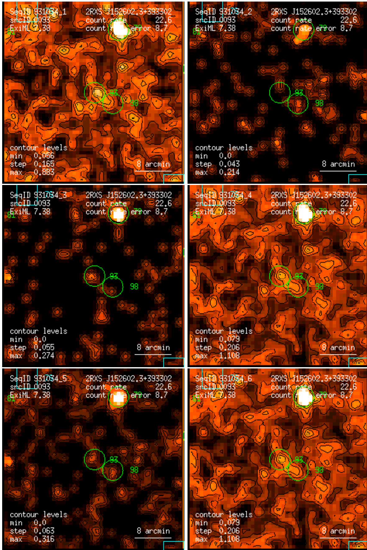
Figure 93: RASS 931034: detection 0093: band rate images, Gaussian filter: (1) PSPC channels 11 – 41, (2) 52 – 90, (3) 91 – 201, (4) 11 – 235, (5) 52 – 201, (6) 11 – 201. Broad band rates in counts/ks. Band rate contour levels in counts/ks/arcmin 2 .
