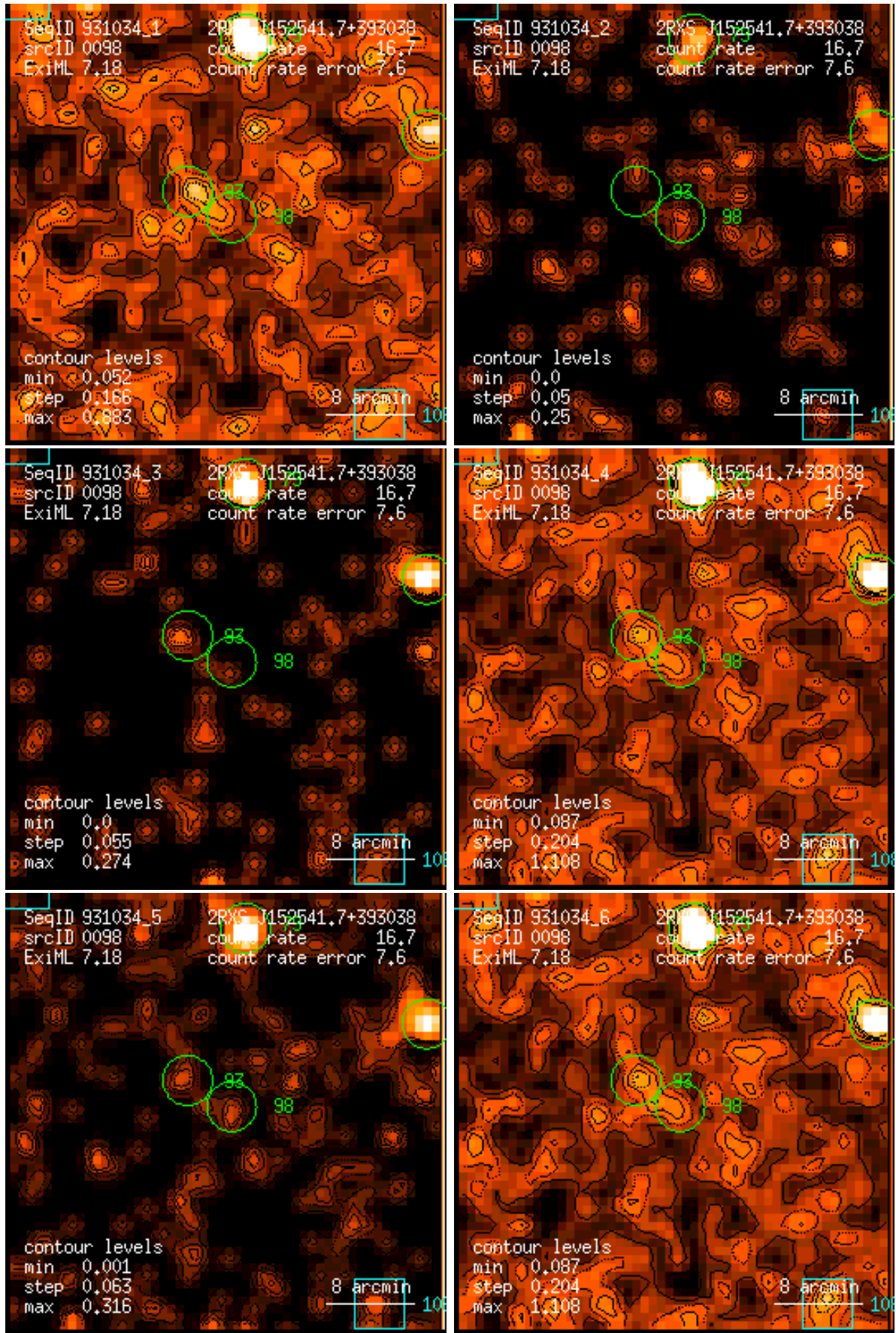
Figure 98: RASS 931034: detection 0098: band rate images, Gaussian filter: (1) PSPC channels 11 – 41, (2) 52 – 90, (3) 91 – 201, (4) 11 – 235, (5) 52 – 201, (6) 11 – 201. Broad band rates in counts/ks. Band rate contour levels in counts/ks/arcmin 2 .
