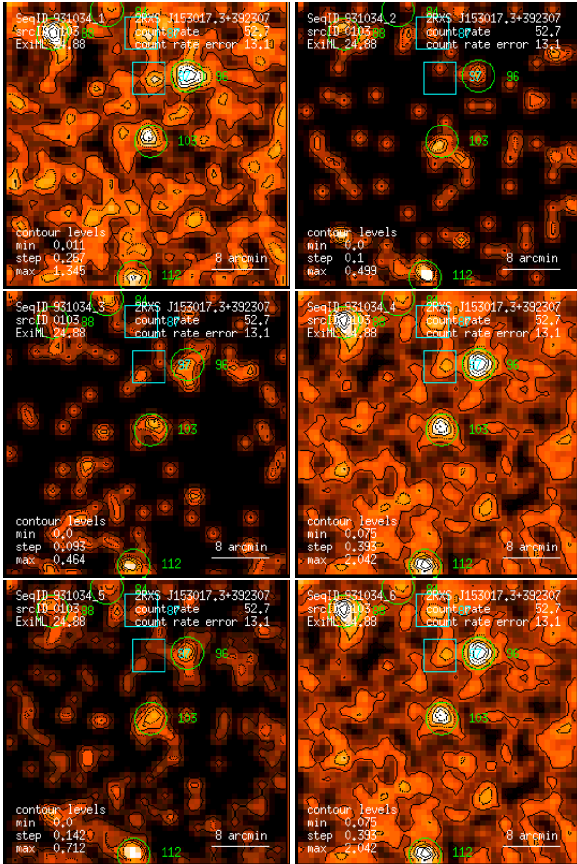
Figure 103: RASS 931034: detection 0103: band rate images, Gaussian filter: (1) PSPC channels 11 – 41, (2) 52 – 90, (3) 91 – 201, (4) 11 – 235, (5) 52 – 201, (6) 11 – 201. Broad band rates in counts/ks. Band rate contour levels in counts/ks/arcmin 2 .
