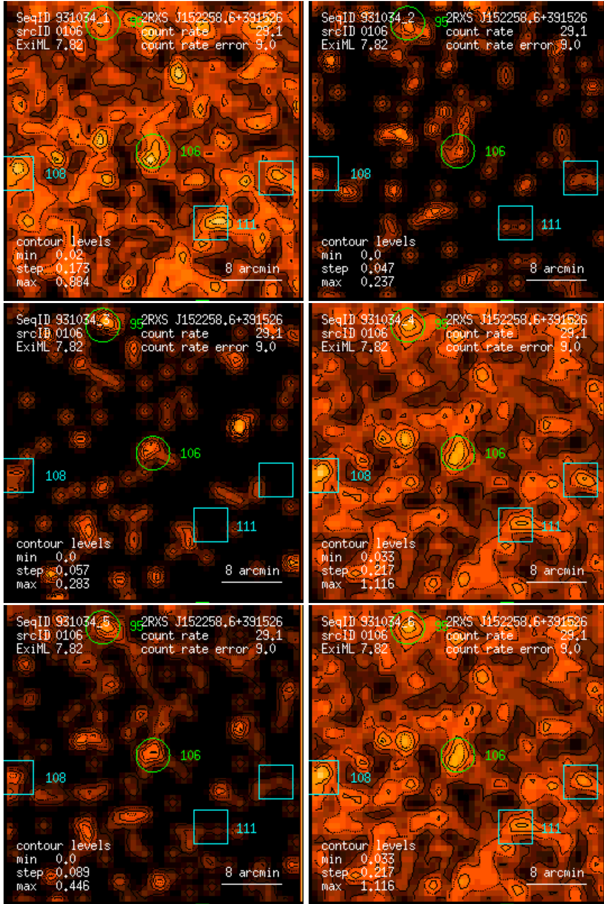
Figure 106: RASS 931034: detection 0106: band rate images, Gaussian filter: (1) PSPC channels 11 – 41, (2) 52 – 90, (3) 91 – 201, (4) 11 – 235, (5) 52 – 201, (6) 11 – 201. Broad band rates in counts/ks. Band rate contour levels in counts/ks/arcmin 2 .
