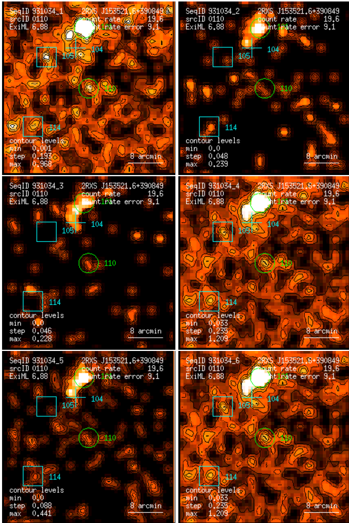
Figure 110: RASS 931034: detection 0110: band rate images, Gaussian filter: (1) PSPC channels 11 – 41, (2) 52 – 90, (3) 91 – 201, (4) 11 – 235, (5) 52 – 201, (6) 11 – 201. Broad band rates in counts/ks. Band rate contour levels in counts/ks/arcmin 2 .
