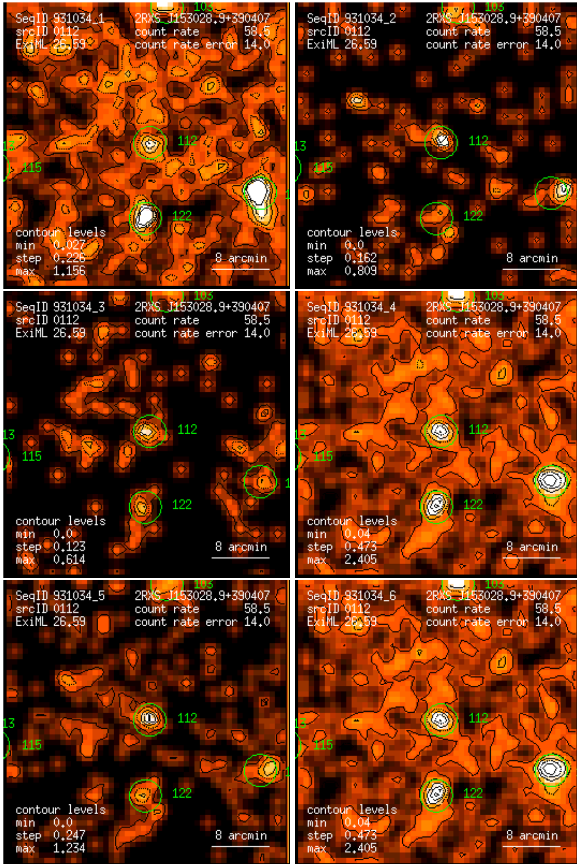
Figure 112: RASS 931034: detection 0112: band rate images, Gaussian filter: (1) PSPC channels 11 – 41, (2) 52 – 90, (3) 91 – 201, (4) 11 – 235, (5) 52 – 201, (6) 11 – 201. Broad band rates in counts/ks. Band rate contour levels in counts/ks/arcmin 2 .
