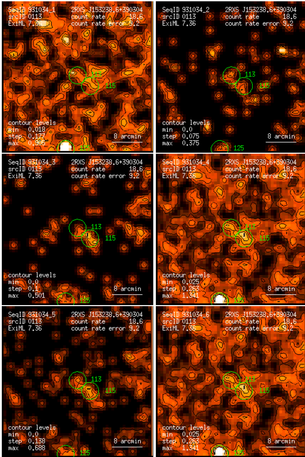
Figure 113: RASS 931034: detection 0113: band rate images, Gaussian filter: (1) PSPC channels 11 – 41, (2) 52 – 90, (3) 91 – 201, (4) 11 – 235, (5) 52 – 201, (6) 11 – 201. Broad band rates in counts/ks. Band rate contour levels in counts/ks/arcmin 2 .
