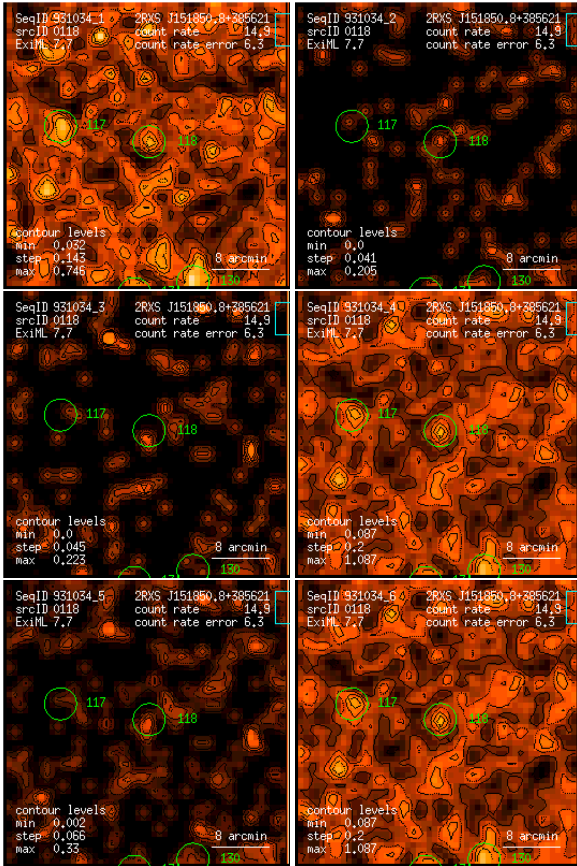
Figure 118: RASS 931034: detection 0118: band rate images, Gaussian filter: (1) PSPC channels 11 – 41, (2) 52 – 90, (3) 91 – 201, (4) 11 – 235, (5) 52 – 201, (6) 11 – 201. Broad band rates in counts/ks. Band rate contour levels in counts/ks/arcmin 2 .
