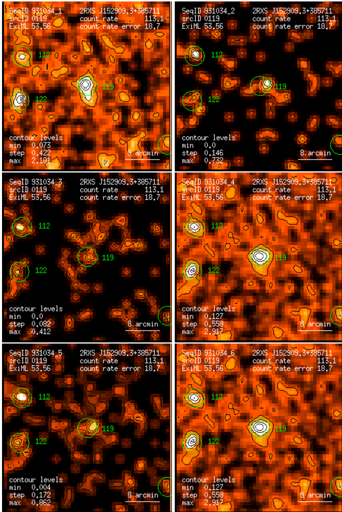
Figure 119: RASS 931034: detection 0119: band rate images, Gaussian filter: (1) PSPC channels 11 – 41, (2) 52 – 90, (3) 91 – 201, (4) 11 – 235, (5) 52 – 201, (6) 11 – 201. Broad band rates in counts/ks. Band rate contour levels in counts/ks/arcmin 2 .
