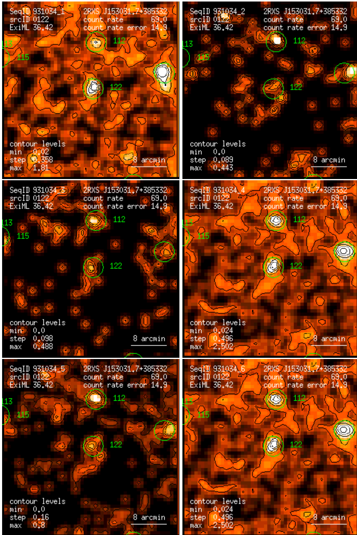
Figure 122: RASS 931034: detection 0122: band rate images, Gaussian filter: (1) PSPC channels 11 – 41, (2) 52 – 90, (3) 91 – 201, (4) 11 – 235, (5) 52 – 201, (6) 11 – 201. Broad band rates in counts/ks. Band rate contour levels in counts/ks/arcmin 2 .
