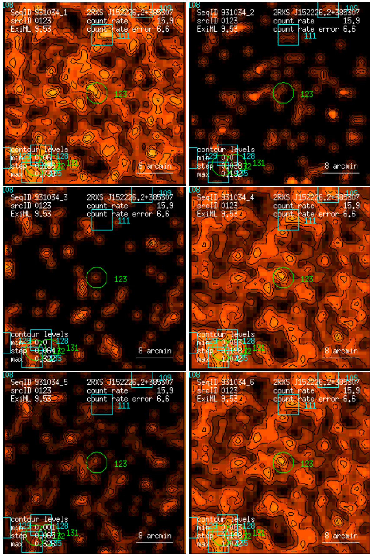
Figure 123: RASS 931034: detection 0123: band rate images, Gaussian filter: (1) PSPC channels 11 – 41, (2) 52 – 90, (3) 91 – 201, (4) 11 – 235, (5) 52 – 201, (6) 11 – 201. Broad band rates in counts/ks. Band rate contour levels in counts/ks/arcmin 2 .
