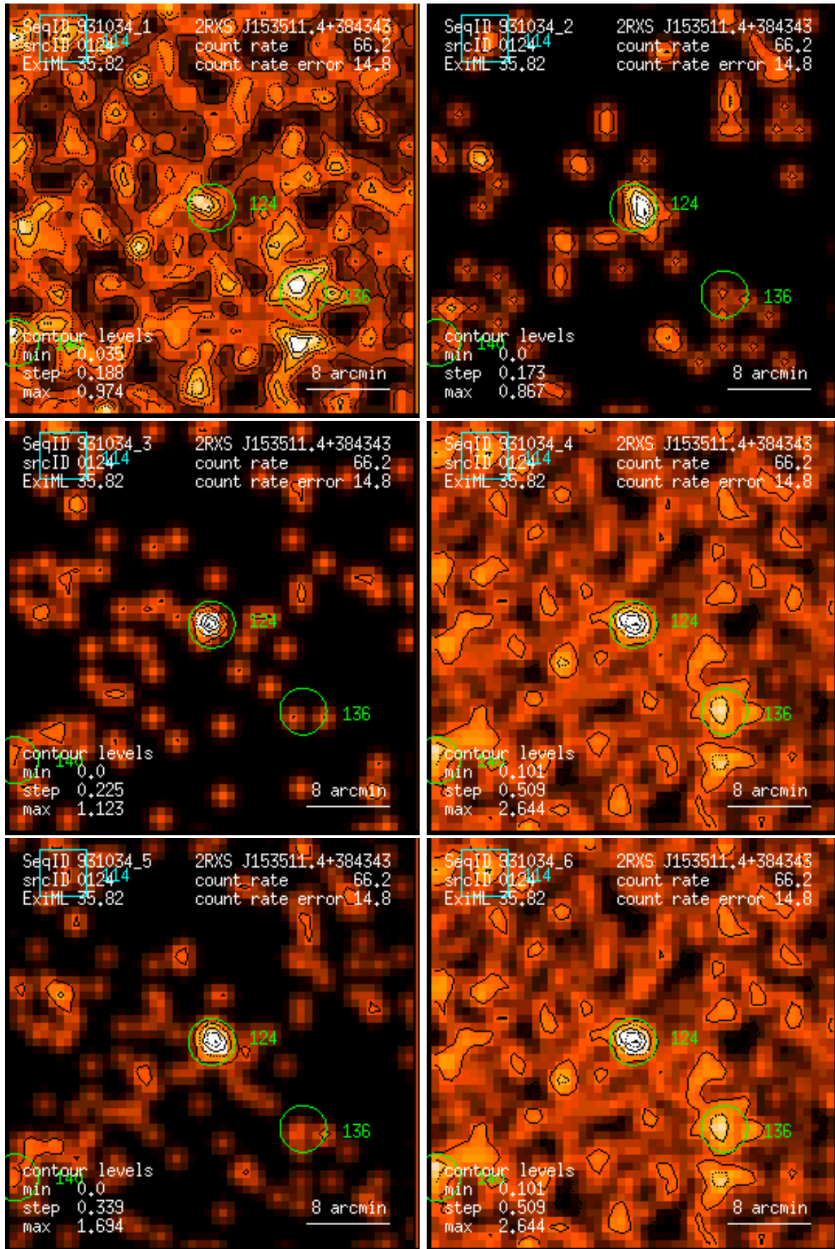
Figure 124: RASS 931034: detection 0124: band rate images, Gaussian filter: (1) PSPC channels 11 – 41, (2) 52 – 90, (3) 91 – 201, (4) 11 – 235, (5) 52 – 201, (6) 11 – 201. Broad band rates in counts/ks. Band rate contour levels in counts/ks/arcmin 2 .
