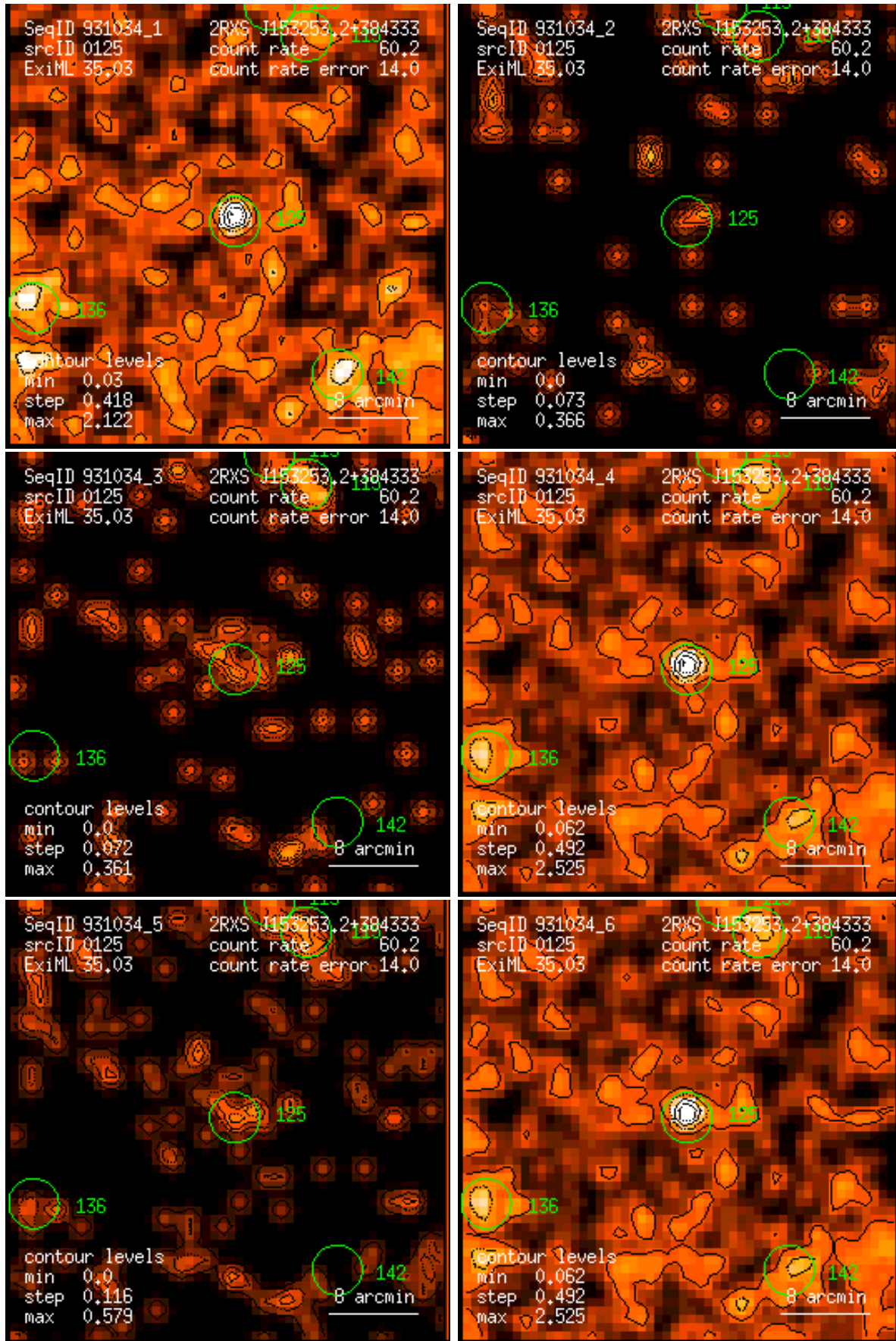
Figure 125: RASS 931034: detection 0125: band rate images, Gaussian filter: (1) PSPC channels 11 – 41, (2) 52 – 90, (3) 91 – 201, (4) 11 – 235, (5) 52 – 201, (6) 11 – 201. Broad band rates in counts/ks. Band rate contour levels in counts/ks/arcmin 2 .
