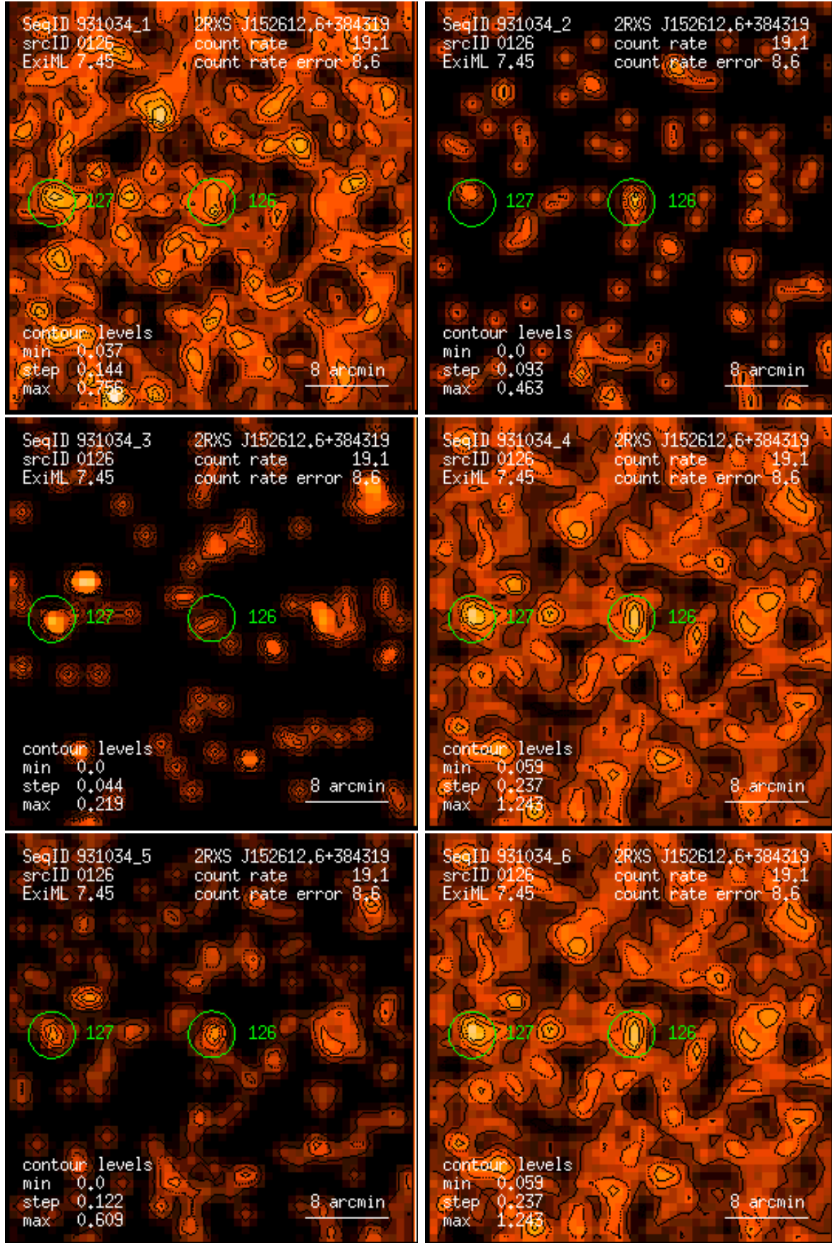
Figure 126: RASS 931034: detection 0126: band rate images, Gaussian filter: (1) PSPC channels 11 – 41, (2) 52 – 90, (3) 91 – 201, (4) 11 – 235, (5) 52 – 201, (6) 11 – 201. Broad band rates in counts/ks. Band rate contour levels in counts/ks/arcmin 2 .
