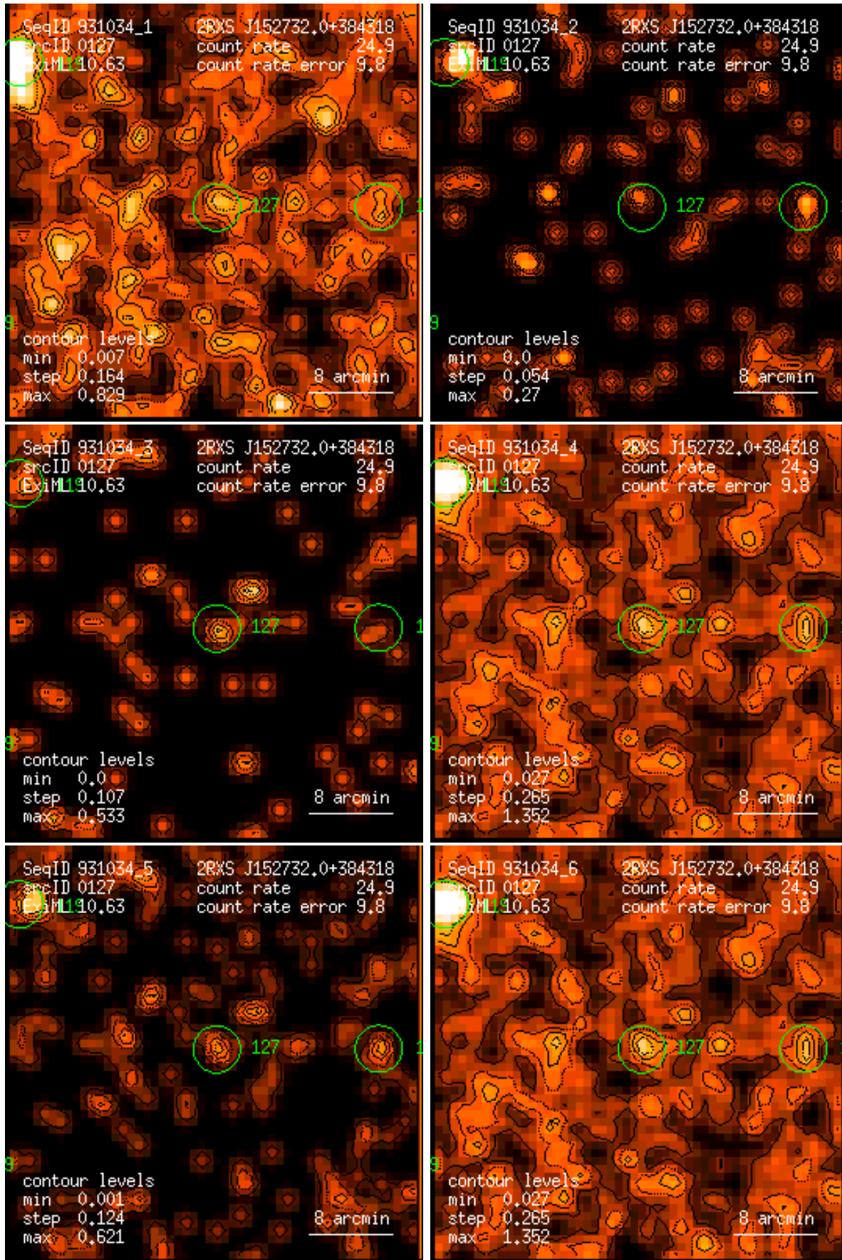
Figure 127: RASS 931034: detection 0127: band rate images, Gaussian filter: (1) PSPC channels 11 – 41, (2) 52 – 90, (3) 91 – 201, (4) 11 – 235, (5) 52 – 201, (6) 11 – 201. Broad band rates in counts/ks. Band rate contour levels in counts/ks/arcmin 2 .
