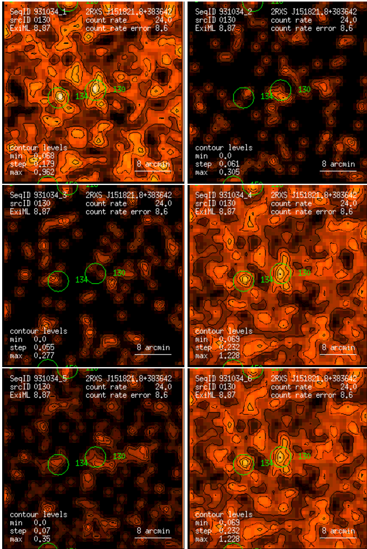
Figure 130: RASS 931034: detection 0130: band rate images, Gaussian filter: (1) PSPC channels 11 – 41, (2) 52 – 90, (3) 91 – 201, (4) 11 – 235, (5) 52 – 201, (6) 11 – 201. Broad band rates in counts/ks. Band rate contour levels in counts/ks/arcmin 2 .
