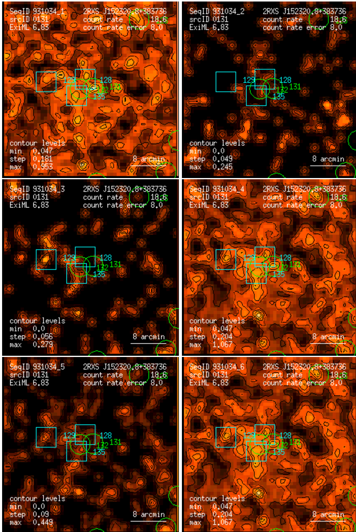
Figure 131: RASS 931034: detection 0131: band rate images, Gaussian filter: (1) PSPC channels 11 – 41, (2) 52 – 90, (3) 91 – 201, (4) 11 – 235, (5) 52 – 201, (6) 11 – 201. Broad band rates in counts/ks. Band rate contour levels in counts/ks/arcmin 2 .
