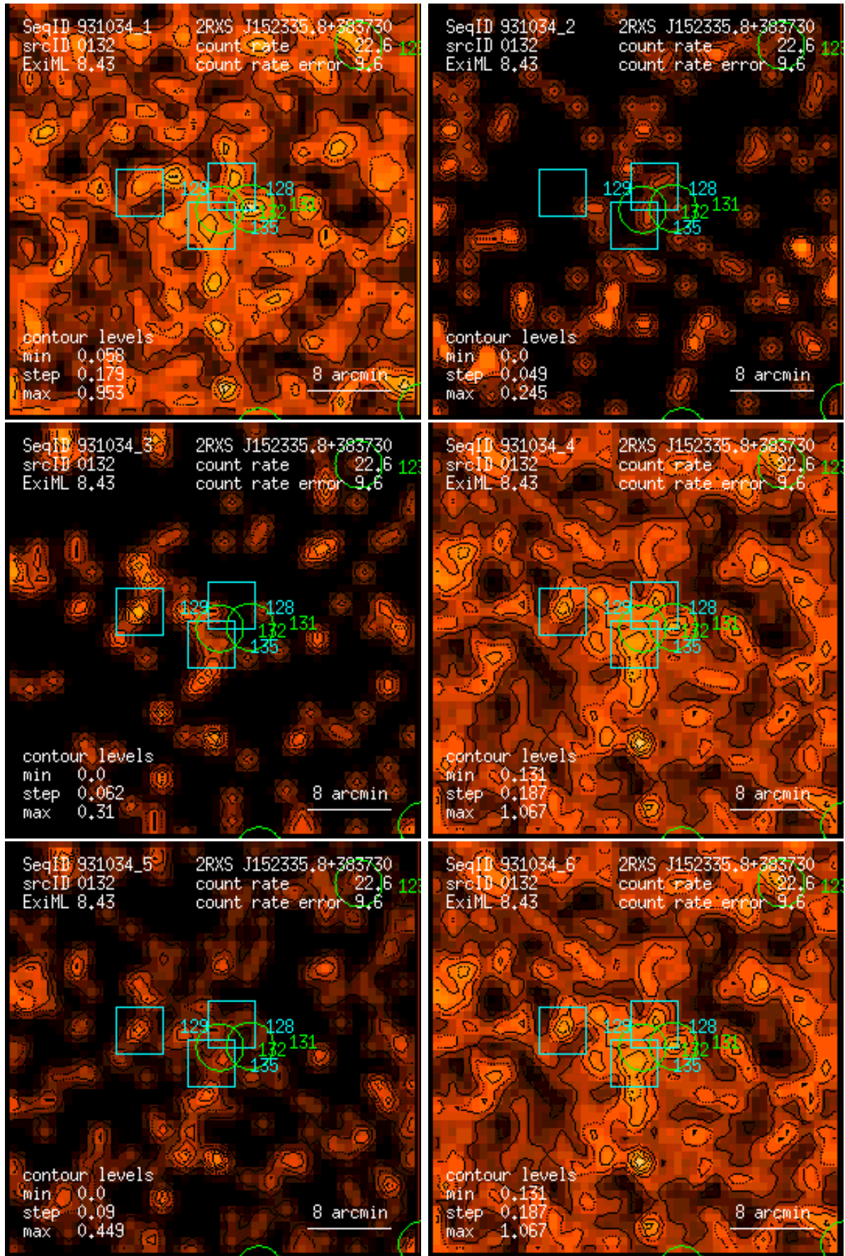
Figure 132: RASS 931034: detection 0132: band rate images, Gaussian filter: (1) PSPC channels 11 – 41, (2) 52 – 90, (3) 91 – 201, (4) 11 – 235, (5) 52 – 201, (6) 11 – 201. Broad band rates in counts/ks. Band rate contour levels in counts/ks/arcmin 2 .
