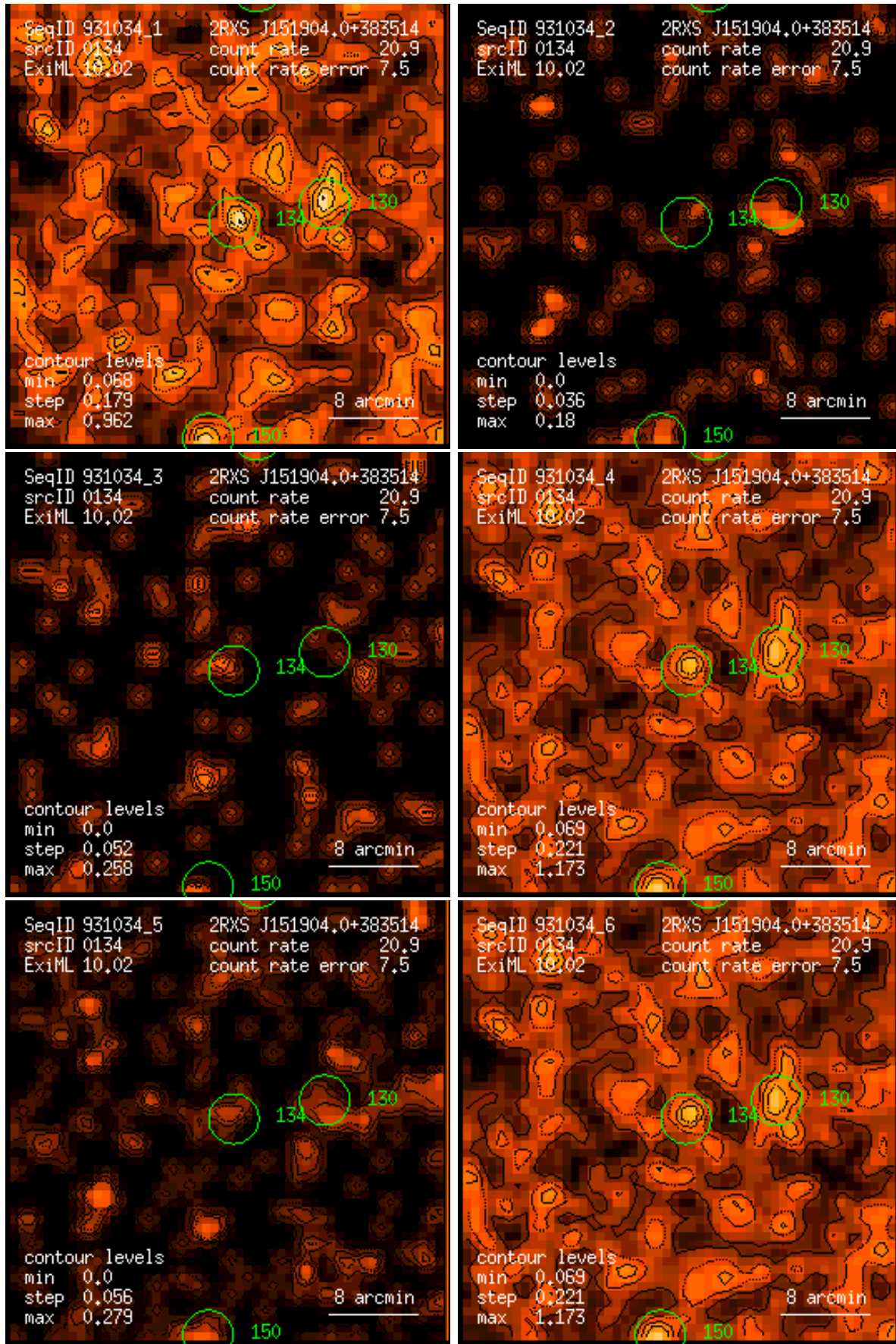
Figure 134: RASS 931034: detection 0134: band rate images, Gaussian filter: (1) PSPC channels 11 – 41, (2) 52 – 90, (3) 91 – 201, (4) 11 – 235, (5) 52 – 201, (6) 11 – 201. Broad band rates in counts/ks. Band rate contour levels in counts/ks/arcmin 2 .
