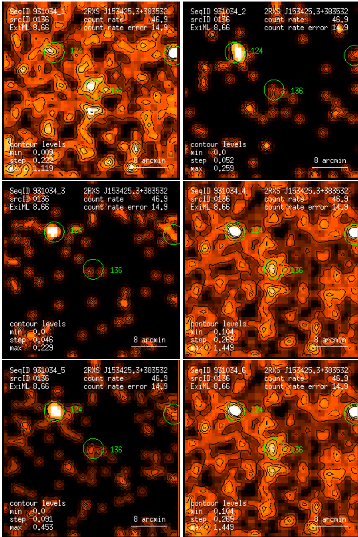
Figure 136: RASS 931034: detection 0136: band rate images, Gaussian filter: (1) PSPC channels 11 – 41, (2) 52 – 90, (3) 91 – 201, (4) 11 – 235, (5) 52 – 201, (6) 11 – 201. Broad band rates in counts/ks. Band rate contour levels in counts/ks/arcmin 2 .
