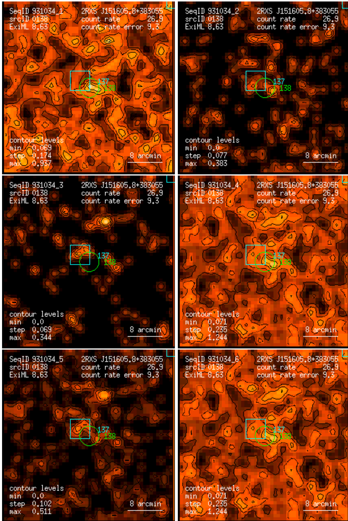
Figure 138: RASS 931034: detection 0138: band rate images, Gaussian filter: (1) PSPC channels 11 – 41, (2) 52 – 90, (3) 91 – 201, (4) 11 – 235, (5) 52 – 201, (6) 11 – 201. Broad band rates in counts/ks. Band rate contour levels in counts/ks/arcmin 2 .
