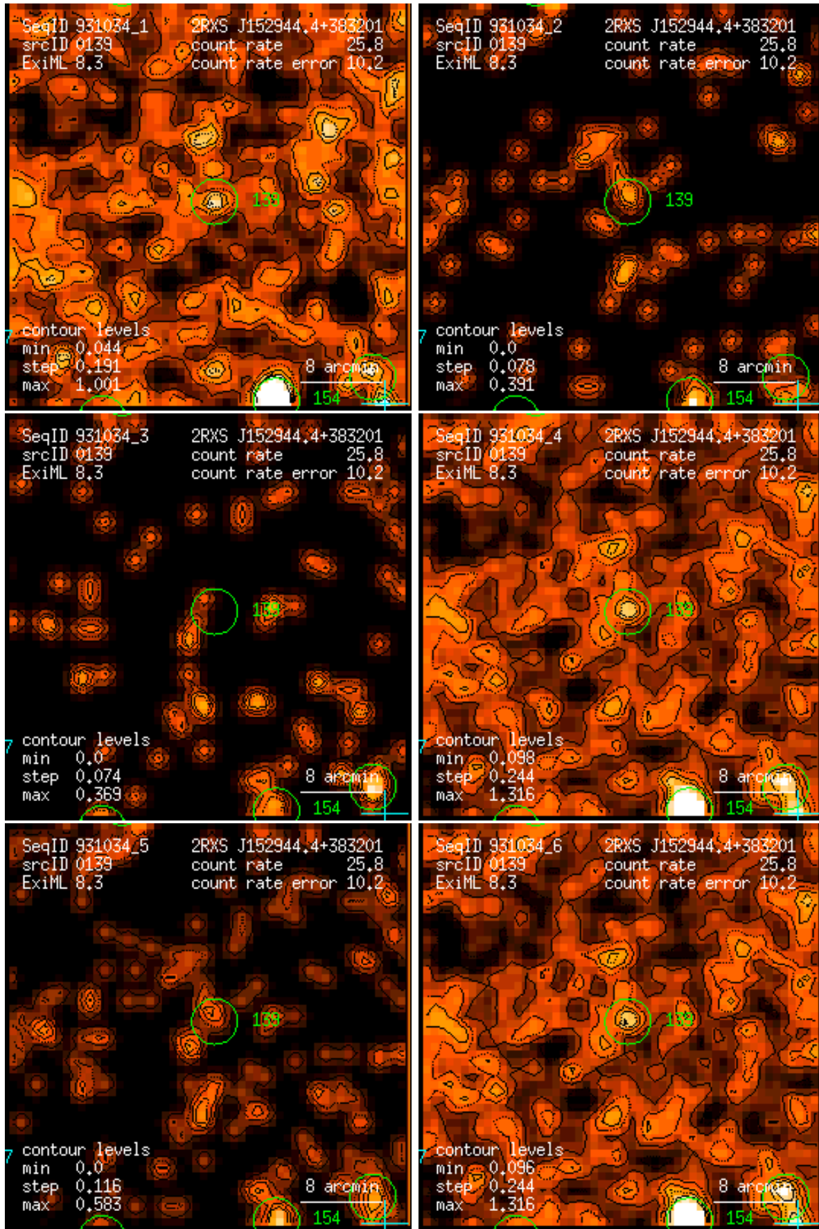
Figure 139: RASS 931034: detection 0139: band rate images, Gaussian filter: (1) PSPC channels 11 – 41, (2) 52 – 90, (3) 91 – 201, (4) 11 – 235, (5) 52 – 201, (6) 11 – 201. Broad band rates in counts/ks. Band rate contour levels in counts/ks/arcmin 2 .
