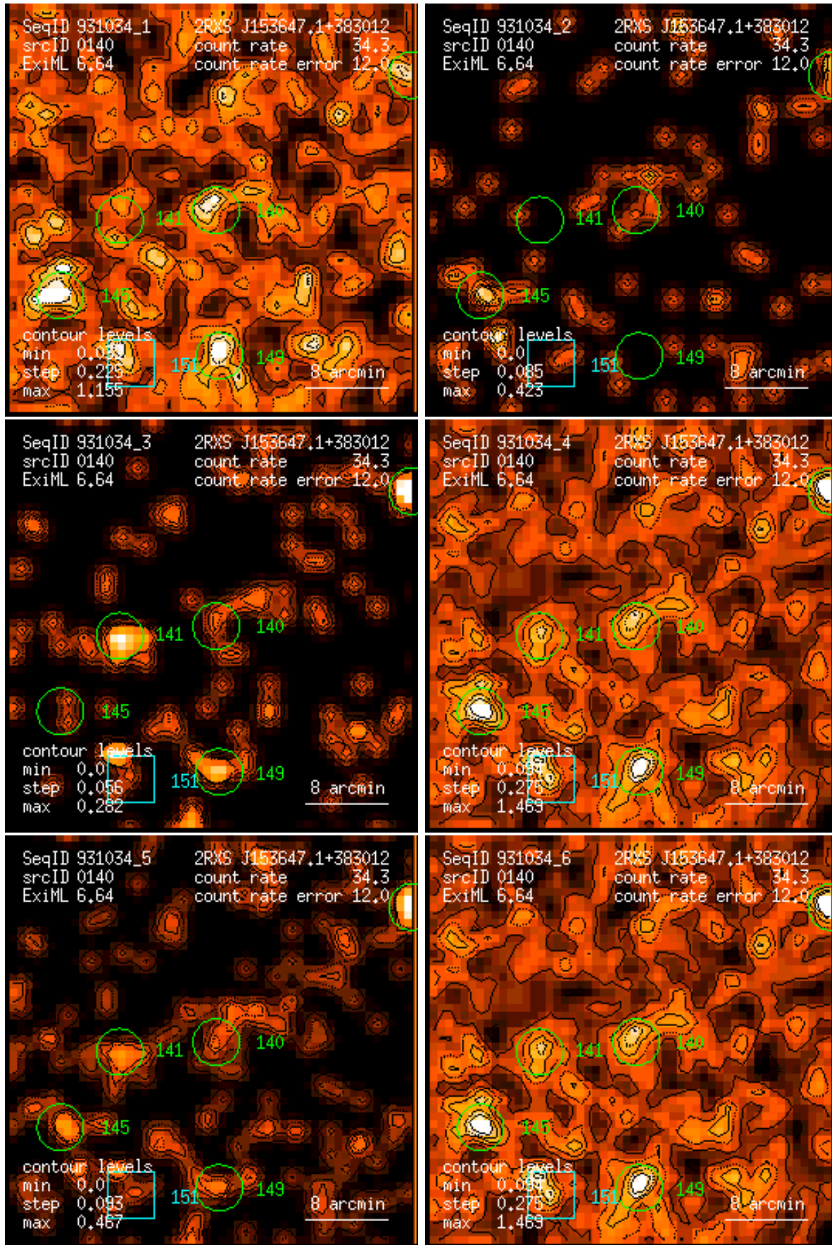
Figure 140: RASS 931034: detection 0140: band rate images, Gaussian filter: (1) PSPC channels 11 – 41, (2) 52 – 90, (3) 91 – 201, (4) 11 – 235, (5) 52 – 201, (6) 11 – 201. Broad band rates in counts/ks. Band rate contour levels in counts/ks/arcmin 2 .
